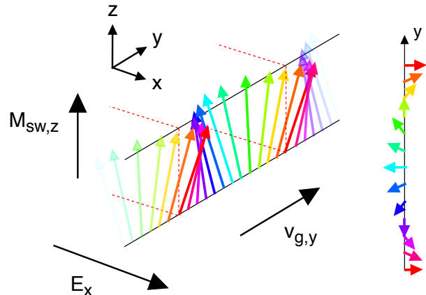
Figure 1. Spin waves in an electric field. The ferromagnet has main magnetization along z . The spin waves are the small oscillations of the magnetization vector around the z axis (top view at the right hand side). The magnetic moment current transported by the spin wave is j_{M,yz} = v_{g,y} M_{sw,z} where v_{g,y} is the group velocity (chosen along y ). The static electric field E_x is along x .
