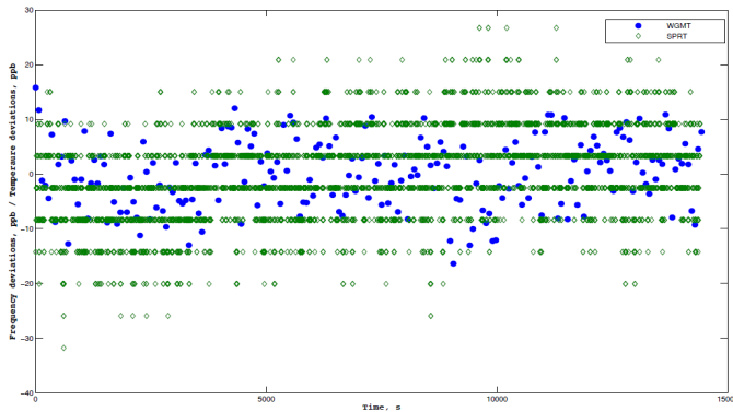
Fig. 13. Comparison of WGMT frequency deviations and SPRT temperature deviations over 4 hours at 60 °C.
