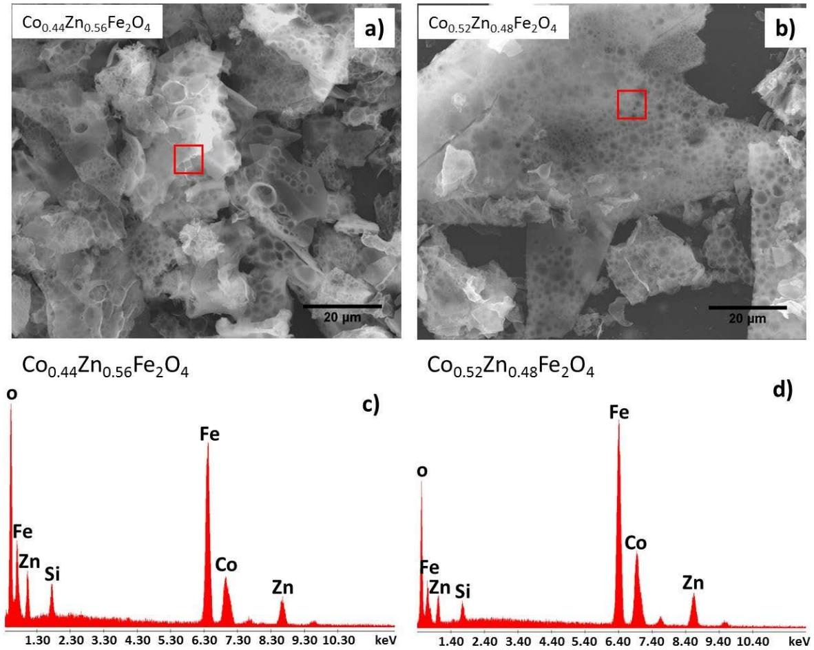
Figure 2: Morphology of the \text{Co}_{0.44}\text{Zn}_{0.56}\text{Fe}_2\text{O}_4 (panel a) and \text{Co}_{0.52}\text{Zn}_{0.48}\text{Fe}_2\text{O}_4 (panel b) ferrite powder samples; EDS spectra of the \text{Co}_{0.44}\text{Zn}_{0.56}\text{Fe}_2\text{O}_4 (panel c) and \text{Co}_{0.52}\text{Zn}_{0.48}\text{Fe}_2\text{O}_4 (panel d) ferrite powder samples. The red squares in the SEM images (panel a and b) represent the analyzed area to obtain the EDS spectra.
