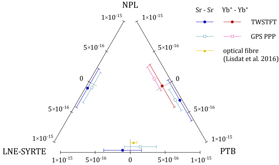
Figure 5. The results of the relative frequency deviation differences for the optical clock comparisons between the three institutes LNE-SYRTE, NPL and PTB, for clocks of the same type. The triangle plot is explained in the text at the beginning of section 4. The result for the fibre comparison is taken from [20].
