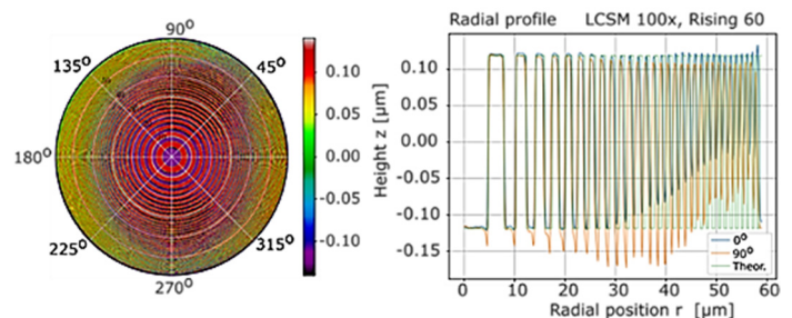
Figure 16. Topography fidelity artefact designed by PTB [65]. Topography data map of the circular chirp pattern (radius of 60 \mu\text{m} ) measured by a commercial laser scanning confocal microscope with a 100 \times objective (left) and its profiles along the orientation of 0 ^\circ and 90 ^\circ (right).
