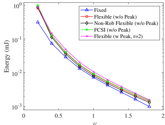
Fig. 7. Example 2: Harvested energy at the relay node versus \nu at P_s = 10 dBm and \sigma_e^2 = 0.1 .
