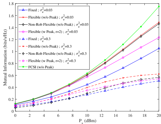
Fig. 8. Example 3: MI versus P_s with \nu = 1 .
