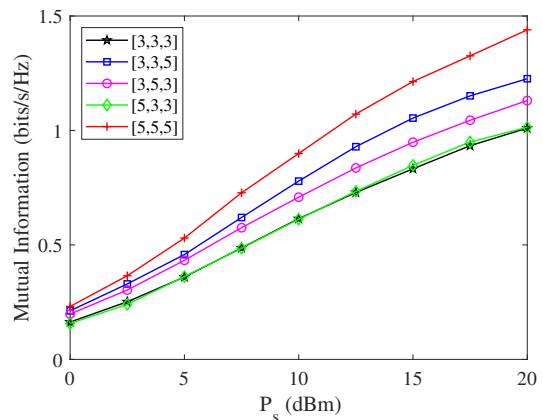
Fig. 10. Example 5: MI versus P_s for robust transceiver design with peak power constraint at various [N_S, N_R, N_D] , r = 2 , \nu = 1 , and \sigma_e^2 = 0.15 .
