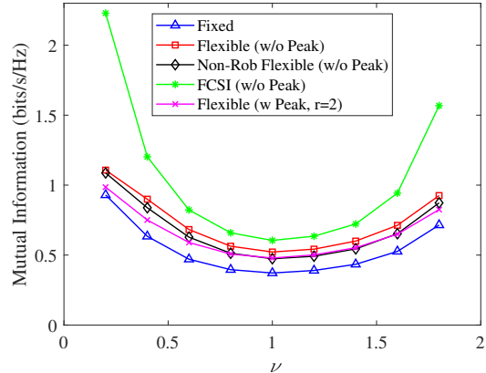
Fig. 6. Example 2: MI versus \nu at P_s = 10 dBm and \sigma_e^2 = 0.1 .
