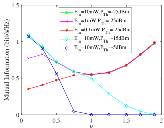
Fig. 11. Example 6: MI versus \nu for robust transceiver design with fixed power scheme at different P_{Th} and E_m with P_s = 15 dBm and \sigma_e^2 = 0.1 .
