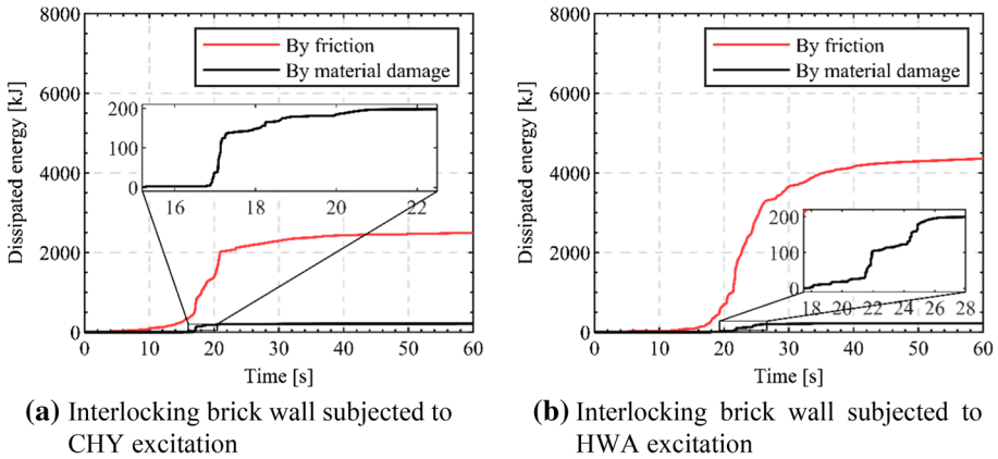
Fig. 28 Energy dissipated by different mechanisms under pulse-like and non-pulse-like ground motions
