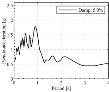
(e) CHY acceleration response spectra
