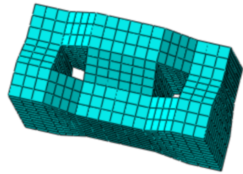
(b) Meshing of one brick
