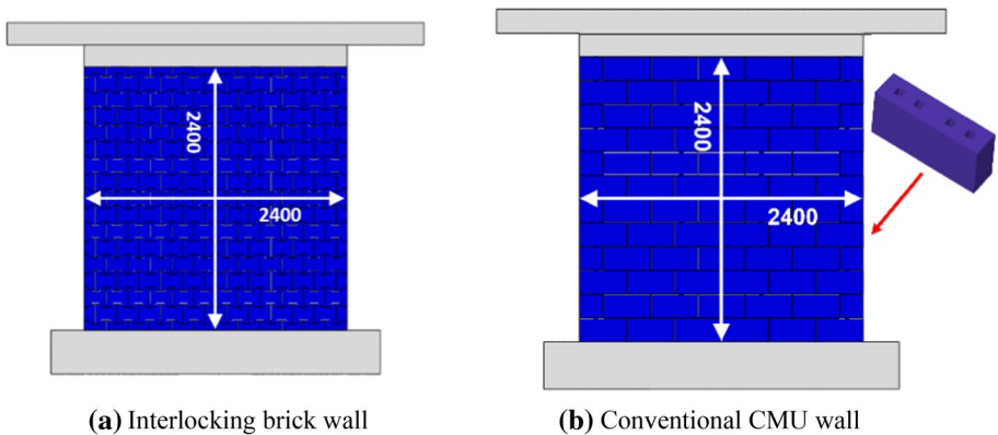
Fig. 14 Full-scale models of the interlocking brick wall and the conventional CMU wall (unit: mm)
