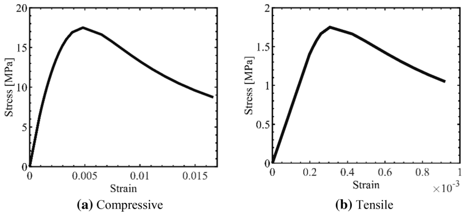
Fig. 6 Stress–strain curves of the brick material
