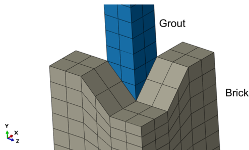
(g) Node position coincidence between the grout and the brick
