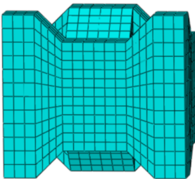
(e) Brick meshing – back view
