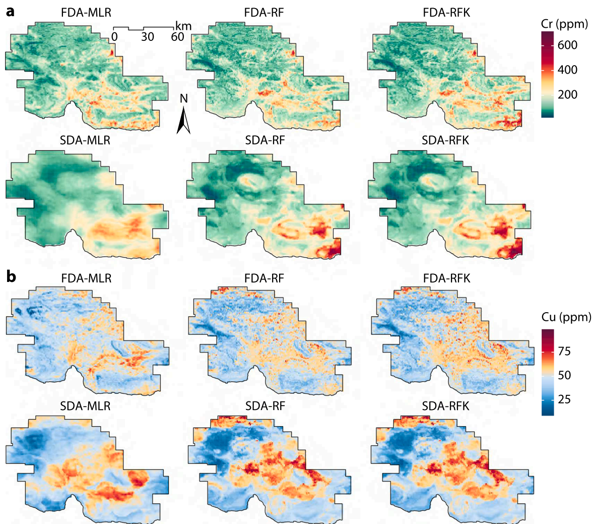
Fig. 7. Spatial predictions of trace elements, Cr (a) and Cu (b), in the study area using the FDA and SDA models.
