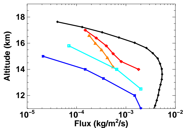
Fig. 9. Mass flux estimates based on \text{O}_3 (red diamonds) and CO (orange triangles) budgets (Dessler, 2002), cloud imagery (cyan squares; Gettelman et al., 2002), and cloud-resolving simulation from Küpper et al. (2004) (blue asterisks) and this work (black crosses).
