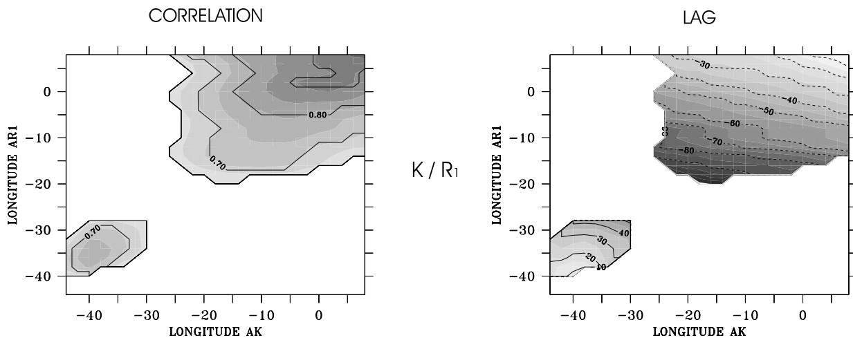
Figure 13. Lag correlation along the equator between K and R_1 coefficients for the second baroclinic mode: (left) correlation greater than 0.6 is represented (CI is 0.1) and (right) lag of maximum correlation is displayed (unit is days, and CI is 10 days).
