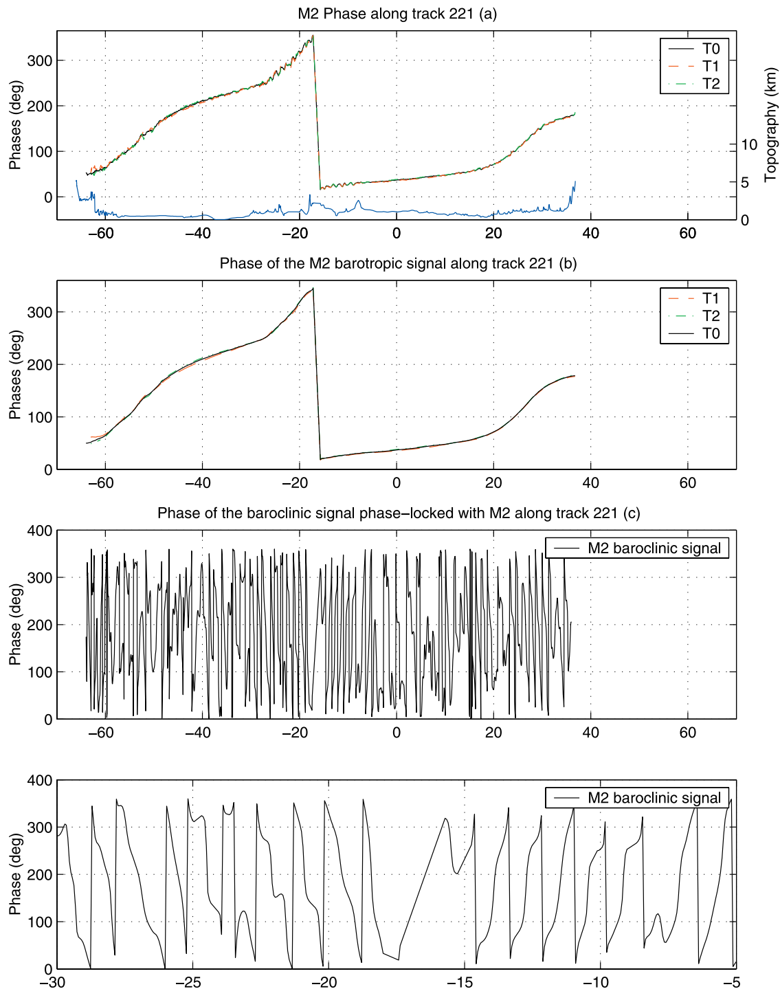
Figure 3. Phase of the barotropic and baroclinic signals along track 221 (over the Tahiti area). T0 is full T/P time series (1993–1999); T1 is first 3 years of T/P data (1993–1995); T2 is last 3 and a half years of T/P data (mid 1996–1999). (a) M_2 phase deduced from along-track harmonic analysis, bottom topography in blue. (b) Phase of the M_2 barotropic signal after low-pass filtering and variability of this barotropic signal (right scale). (c) Phase of the M_2 baroclinic signal with a zoom on the latitudes 30^\circ\text{S} to 5^\circ\text{S} .
