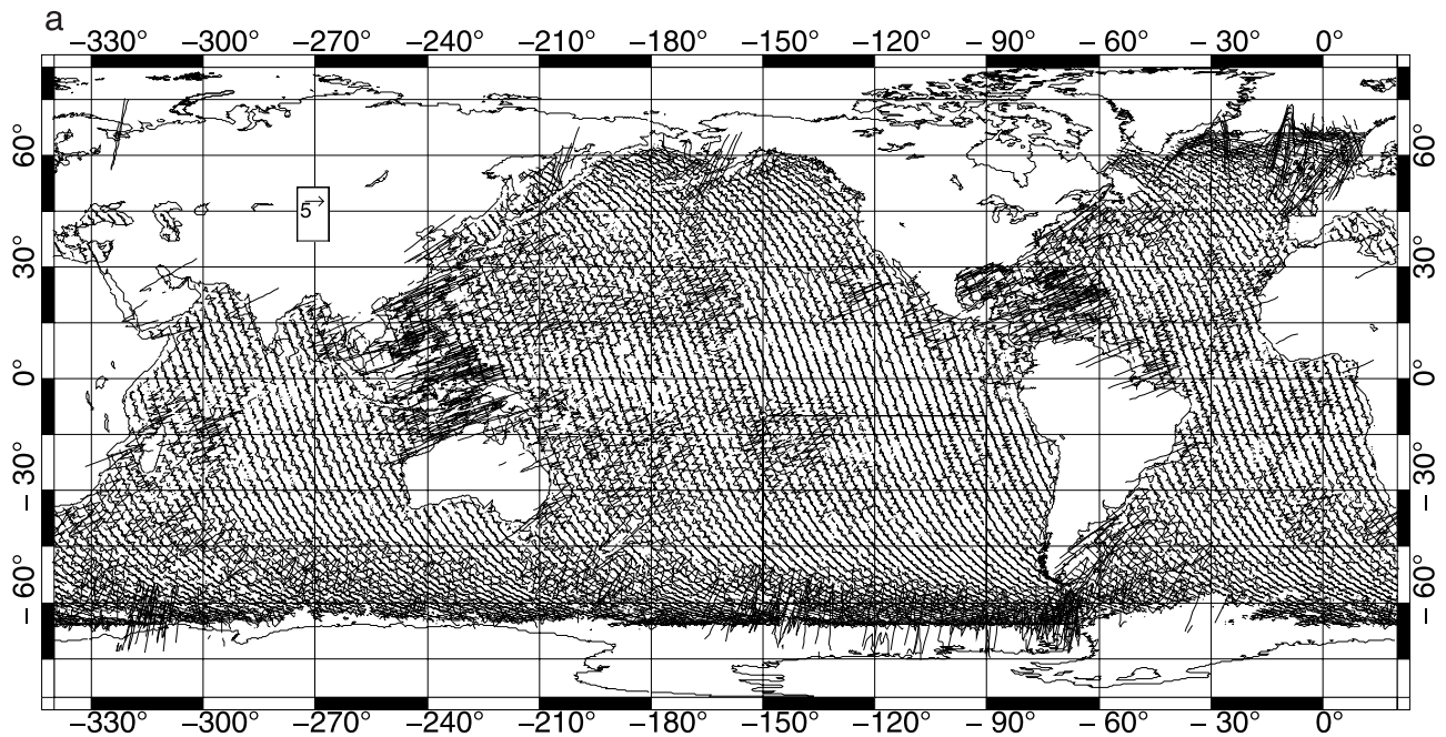
Figure 5. Global charts of the M_2 baroclinic signal deduced from T/P altimetry. (a) M_2 baroclinic amplitude along T/P descending tracks in centimeters. (b) Variability of this M_2 baroclinic signal in centimeters. (c) Signal-to-noise ratio for the M_2 baroclinic tide deduced from T/P altimetry.
