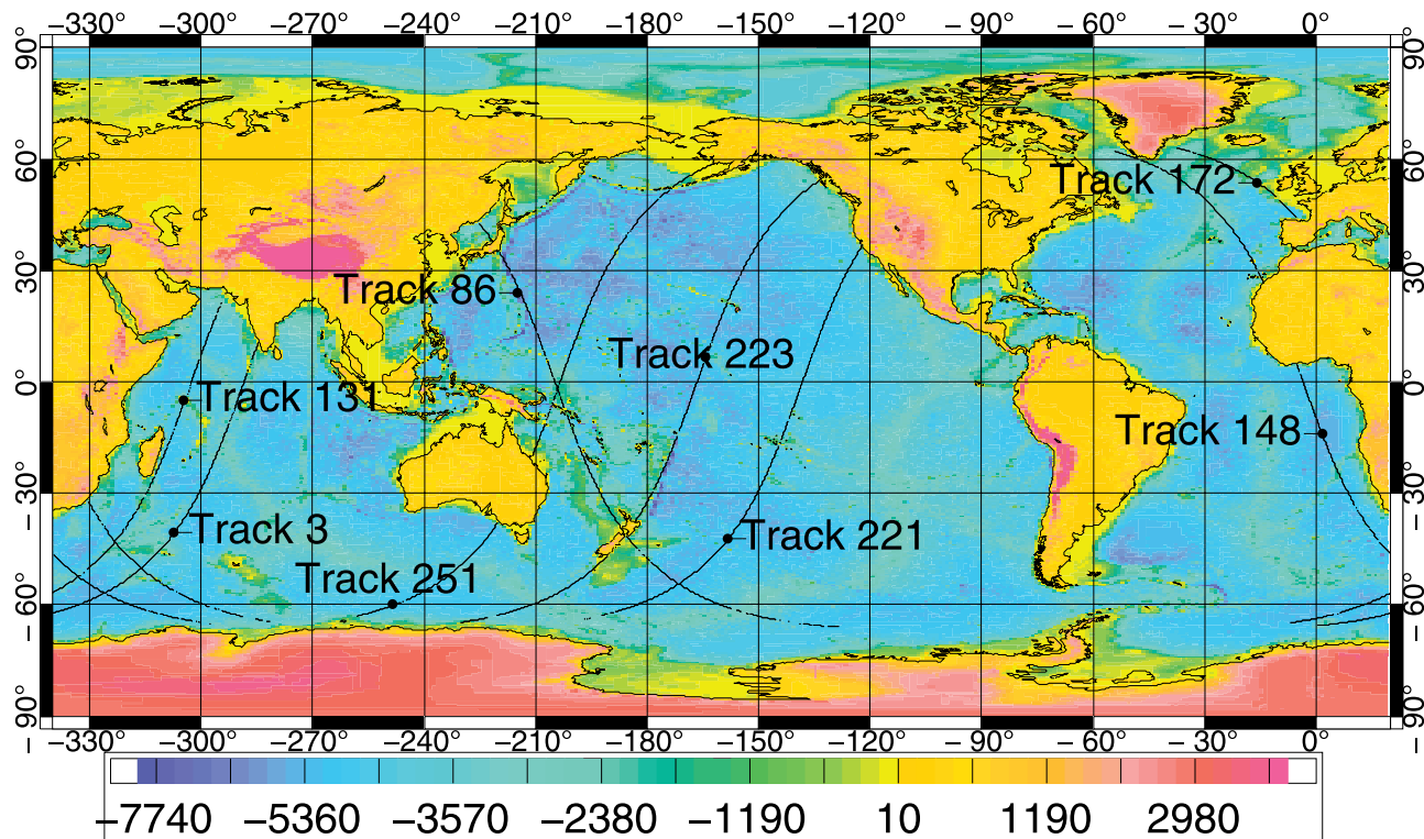
Figure 1. Location of the studied TOPEX/Poseidon (T/P) tracks, overlaying the ocean bottom bathymetry (scale in meters).
