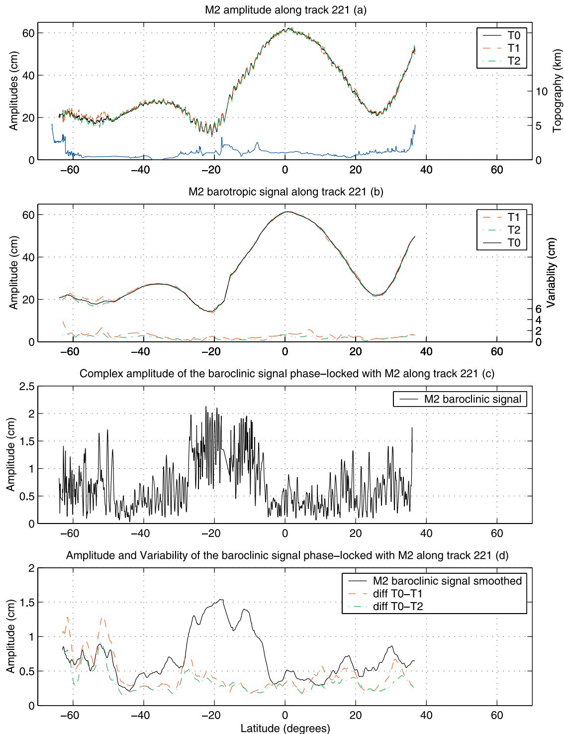
Figure 2. Amplitude of the barotropic and baroclinic signals along track 221 (over the Tahiti area). T0 is full T/P time series analyzed (1993–1999); T1 is first 3 years of T/P data (1993–1995); T2 is last 3 and a half years of T/P data (mid 1996–1999). (a) M_2 amplitude deduced from along-track harmonic analysis, bottom topography in blue. (b) Amplitude of the M_2 barotropic signal after low-pass filtering and variability of this barotropic signal (right scale). (c) Complex amplitude of the M_2 baroclinic signal. (d) Low-pass-filtered complex amplitude of the M_2 baroclinic signal and variability of this baroclinic signal.
