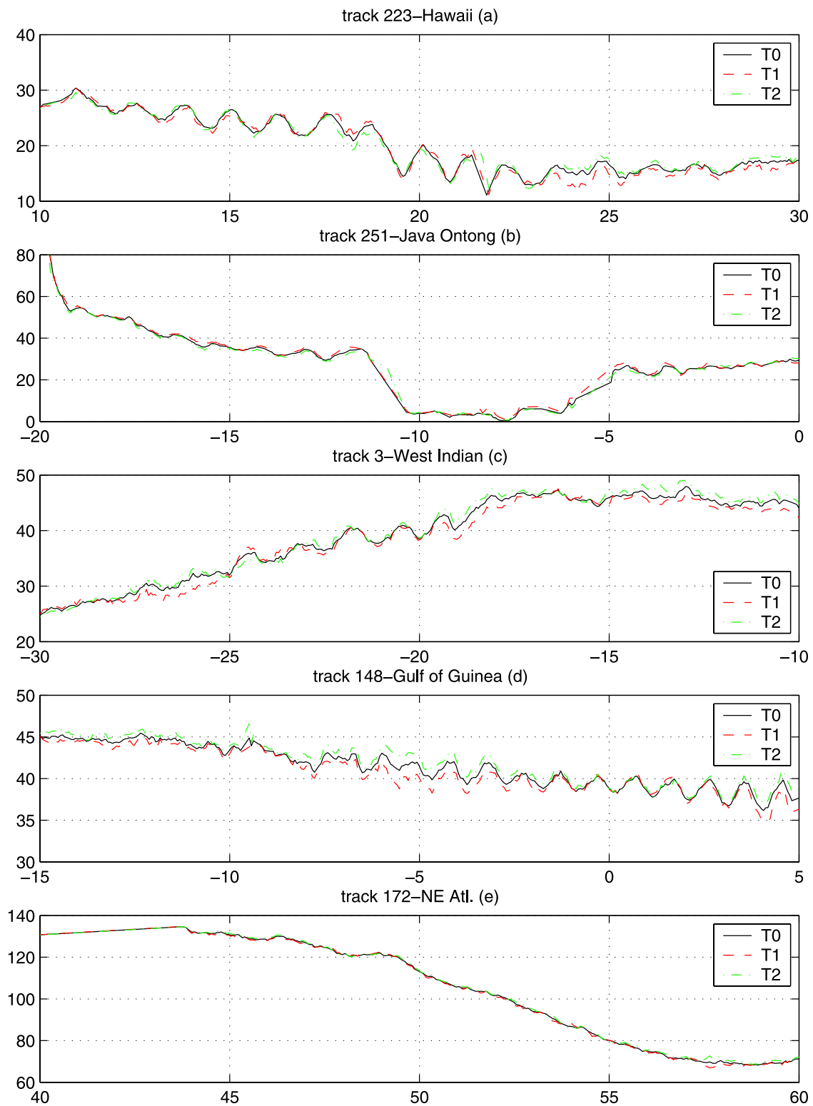
Figure 6. Zoom on five areas where internal wave signatures appear in T/P measurements. Amplitude of the along-track M_2 signal (barotropic plus baroclinic) is in centimeters. (a) Track 223 over the Hawaii chain. (b) Track 251 over the Java-Ontong plateau. (c) Track 3 over the west Indian Ocean. (d) Track 148 over the Gulf of Guinea. (e) Track 172 in the northeast Atlantic.
