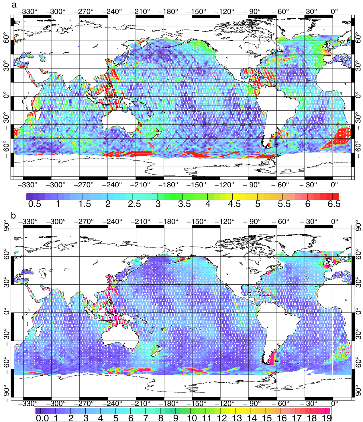
Figure 4. Global charts of the M_2 barotropic signal deduced from T/P altimetry. (a) Variability of this M_2 barotropic signal in centimeters. (b) Amplitude of the complex difference between the M_2 altimetric map and the FES 2002 M_2 wave.
