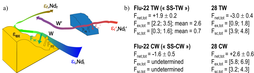
Figure 5. (a) Schematic description of the boundary exchange principle. It illustrates the Nd evolution of a water mass along its transit, initially characterized by an isotopic composition (IC) \epsilon_i and a concentration Nd_i . Each arrow represents a water mass and the color code refers to the IC of each element (margin or water mass). In the box model, two processes can change these initial Nd parameters \epsilon_i (blue) and Nd_i : (i) boundary exchange with a continental margin characterized by a different IC \epsilon_{ex} (yellow), (ii) mixing with a water mass characterized by different Nd parameters, \epsilon'_i (red) and [Nd]'_i . The boundary exchange is defined by two fluxes: the Nd flux supplied by the margin F_{ex} that modifies the IC of the water mass (green), and the Nd flux removed from the water mass toward the sediment F_{sc} that balances the concentration budget. The total net flux is defined as F_{net,tot} = F_{ex,tot} - F_{sc,tot} = F_{ex} + F'_{ex} - F_{sc} - F'_{sc} . W and W' are the transport of the water masses determined by the Lagrangian analysis. The output values of the box model refer to the resulting water mass Nd parameters, \epsilon_f (brown) and Nd_f . (b) Total net fluxes F_{net,tot} calculated from equation (1) and ranges and mean values of F_{ex,tot} and F_{sc,tot} calculated according to the different hypotheses (detailed in section 3.2.2 for station 28 and in the Appendix A for station Flu-22), for each studied water mass (in tons of Nd per year). The estimations of the exchange fluxes occurring along the Flu-22 CW are not reported because they were too variable, precluding us from suggesting a likeable estimation.
