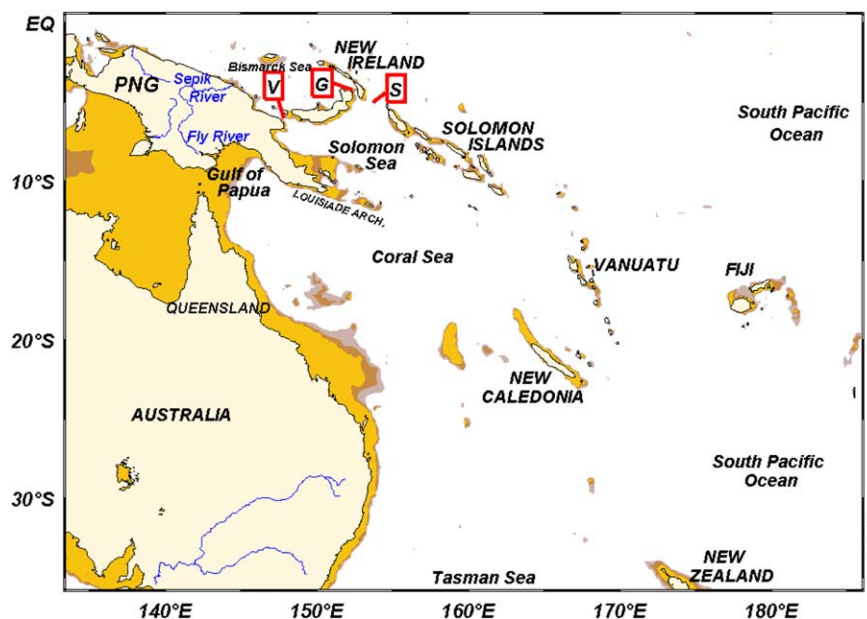
Figure 1. Reference map of the countries, seas, straits, and rivers mentioned in the text. PNG: Papua New Guinea. Red framed « V », « G », and « S », indicate Vitiaz Strait, St. George's Channel, and Solomon Strait, respectively. The bathymetry shallower than 100 m is colored in yellow, in brown if shallower than 250 m, and in light brown if shallower than 500 m.
