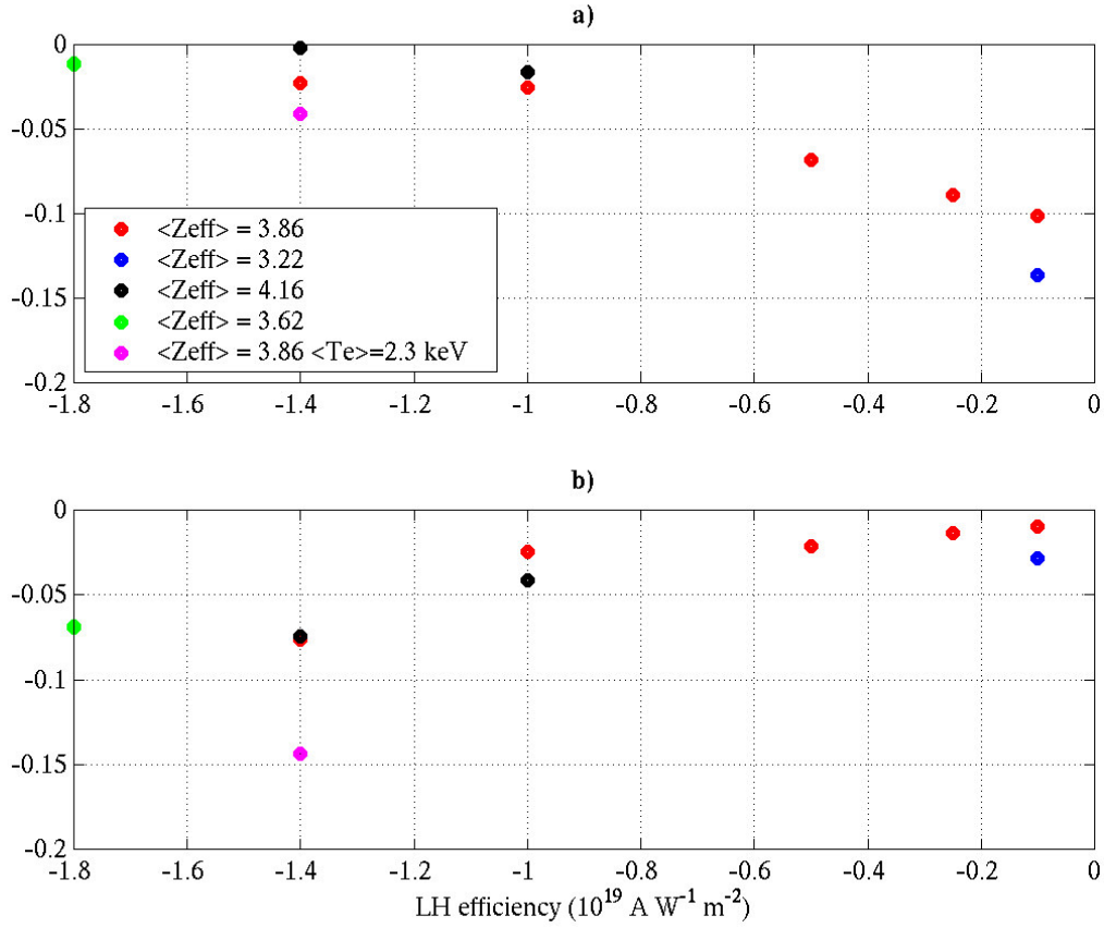
Figure 8 : counter current case, shot #59671, cronos simulation results. a) effect of LH efficiency on the loop voltage ( V_l ) reconstruction. The time average reconstruction of V_l between t=44\text{s} and t=49\text{s} of CRONOS is compared to the experimental one b) same comparison with the self inductance. Effect of the charge effective ( Z_{\text{eff}} ) and the T_e profile is also shown (all the simulation are made with \langle T_e \rangle = 2.4 \text{ keV} except one where the profile was flattened at the edge ( \langle T_e \rangle = 2.3 \text{ keV} )).
