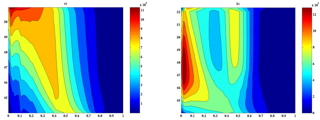
Figure 10 : Contour plot of the total current profile( in A m^{-2} ) deduced from CRONOS a) for the counter current case #59671 b) for the co current case #57326
