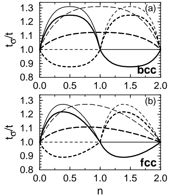
FIG. 3: Effective hopping integrals t_\sigma (in units of t ) as a function of the band filling n of an s band for: (a) bcc and (b) fcc lattices. Different lines refer to: PM phase (long dashed lines), t_1/t (full lines) and t_1/t (dashed lines) in the SF phase (stable at sufficiently large U , see Fig. 2). The parameters are: V = 0.15W ( W = 16t ), J' = J , and: J = 0 (thin lines), J = 0.03W (heavy lines).
