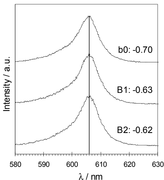
Figure 2. Sensitivity analysis for \text{Cm}(\text{CO}_3)_2^- formation at 25^\circ\text{C} . The value at I = 3 \text{ M} , \log K_3 = 2.08 , was used to calculate the values of \log([\text{CO}_3^{2-}] K_3) written on the figure, while [\text{CO}_3^{2-}] K_3 = [\text{Cm}(\text{CO}_3)_3^{3-}]/[\text{Cm}(\text{CO}_3)_2^-] . These values are similar for the solutions b0, B1 and B2 (Table 1). The spectra are identical although different values were measured for the pH of solutions B1 and B2: -\log[\text{H}^+] = 7.96 and 8.57 , respectively. This evidences no influence of [\text{OH}^-] . Similarly the spectrum for b0 at I = 0.1 \text{ M} is identical to the other ones, which were obtained at higher ionic strength: I = 3 \text{ M} , in agreement with the corresponding ionic strength corrections calculated by using Eqs.(4) and (5).
