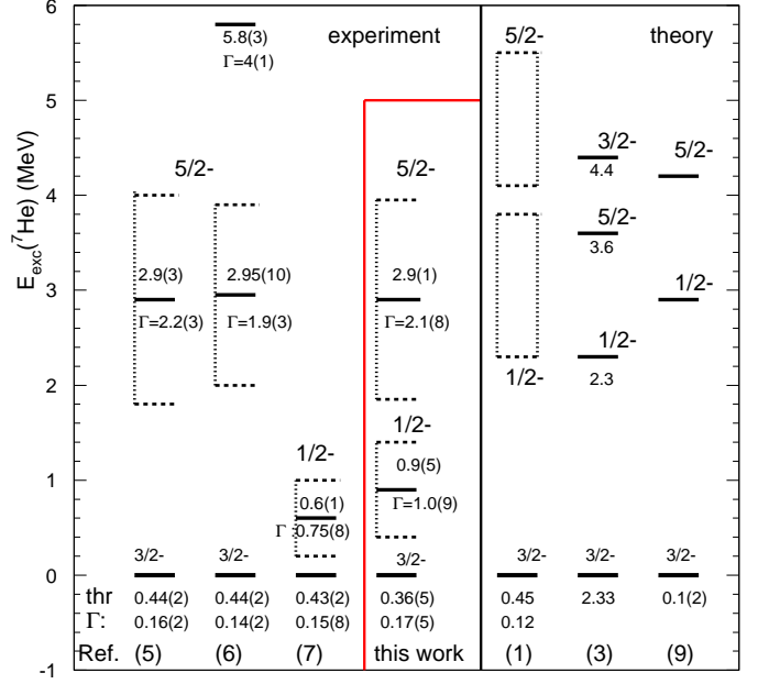
FIG. 8: Experimental and theoretical spectra of {}^7\text{He} . The threshold energy indicated for the models is deduced from the predicted binding energy for {}^7\text{He} and the energies of the excited states are given with respect to the calculated gs.
