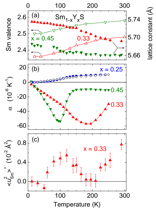
FIG. 2: (Color online) Temperature dependences of lattice properties in \text{Sm}_{1-x}\text{Y}_x\text{S} as obtained from x-ray diffraction measurements: (a) lattice constant for x = 0.33 and 0.45; also plotted is the valence of the same compounds obtained from XAS measurements; (b) thermal expansion coefficient for x = 0.25 , 0.33, and 0.45; data for \text{La}_{0.75}\text{Y}_{0.25}\text{S} are plotted as open circles; (c) relative mean-square displacements of RE ions at T = 10 K for x = 0.33 (see text)
