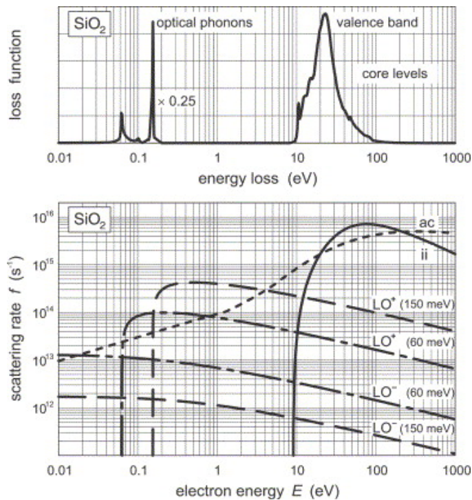
Fig. 1. Dielectric energy loss function (above) and corresponding scattering rates of electrons with longitudinal optical (LO) phonons of energies \hbar\omega_1=150 meV and \hbar\omega_2=60 meV; LO + phonon emission, LO - phonon annihilation; then with acoustic (a.c.) phonons, and due to impact ionization (i.i.) of valence band electrons in SiO 2 corresponding to the dielectric energy loss function above.
