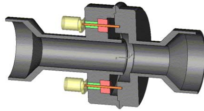
Figure 5 : BPM for the probe beam linac.
