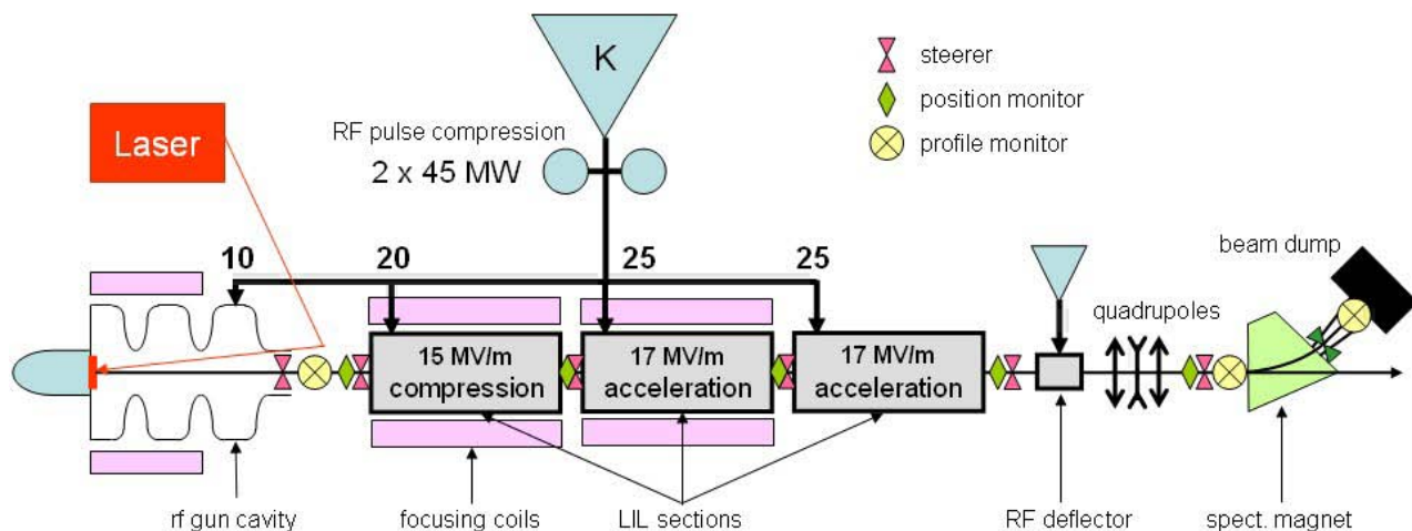
Figure 1: Schematic layout of the probe beam linac (Califes).
