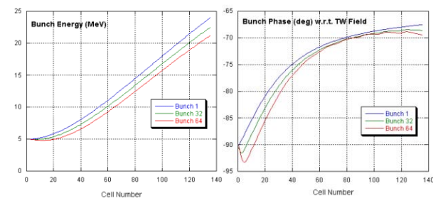
Figure 3 : Bunch energy and phase at the exit of compression section at full current.
