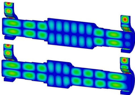
Figure 4: Electric field inside the power phase shifter for two lengths of the widened waveguide.
