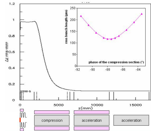
Figure 2 : rms bunch length along the linac and sensitivity to the RF phase (box).
