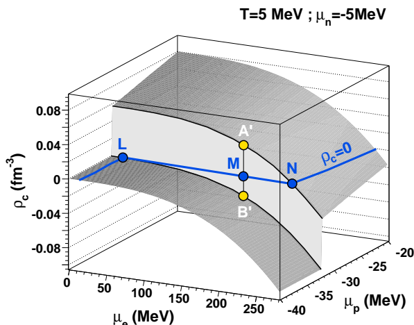
FIG. 2: (Color online) Net charge density \rho_c = -\partial g'/\partial \mu'_c as a function of the proton and electron chemical potential for a neutralized Coulomb system at fixed temperature and neutron chemical potential, with the Sly230a effective interaction. The solid line gives the physical constraint \rho_c = \text{cte} = 0 . The neutralized model presenting a first order phase transition with a \rho_c discontinuity, the physical constraint forces the system to follow the coexistence line, leading to a continuous transition for the physical system.
