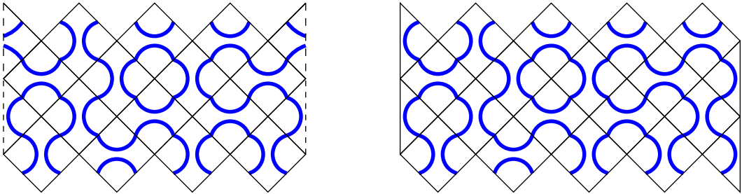
Figure 2: Action of a term in T^2 on a zig-zag row of L plaquettes. The left (resp. right) picture illustrates periodic (resp. free, or reflecting) boundary conditions in the space direction.
