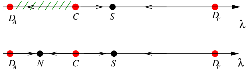
Figure 4: Phase diagram for the loop model (top) and the height model (bottom). The arrows indicate renormalization group flows. The cross-hatching between the new critical point C and the decoupled antiferromagnetic critical point D_A represents the critical phase.
