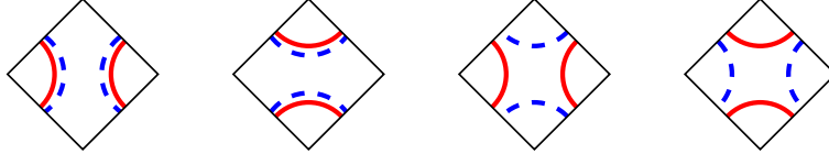
Figure 3: The four configurations at each vertex in the coupled completely packed loop model.
