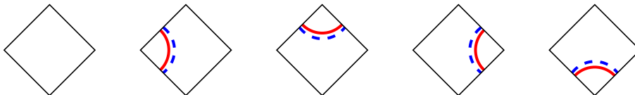
Figure 8: The five additional configurations at each vertex in the dilute loop model.
