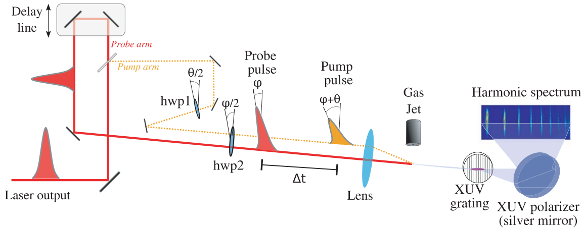
Figure 2. Experimental set-up (see text).
