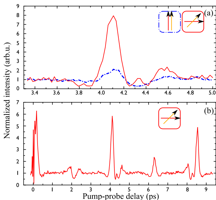
Figure 6. Pump-probe scans in \text{N}_2 , with a pump intensity of 5 \times 10^{13} \text{ W cm}^{-2} and a probe intensity of 1.2 \times 10^{14} \text{ W} \cdot \text{cm}^{-2} . (a) Evolution of the H21 signal as a function of pump-probe delay in two configurations. Conventional configuration (blue): the pump and probe pulse polarizations are parallel and the analyzing waveplate is rotated to maximize the reflection on the polarizer (S polarization). Polarization-resolved spectroscopy (red): the pump-pulse polarization is rotated by 40^\circ with respect to the probe. The analyzing waveplate is rotated so that the probe pulse is P polarized on the polarizer. (b) Evolution of the H19 intensity as a function of pump-probe delay over a full-rotational period of \text{N}_2 , in the polarization resolved spectroscopy configuration.
