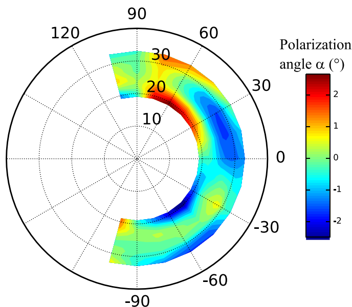
Figure 4. Polarimetry of high harmonic generation in aligned N_2 . The colormap shows the angle \alpha between the laser polarization and the harmonic polarization, in degrees. The radial direction is the harmonic order, from 19 to 33. The polar coordinate corresponds to the molecular alignment angle \theta with respect to the probe laser field ( \theta = 0^\circ is along the horizontal direction).
