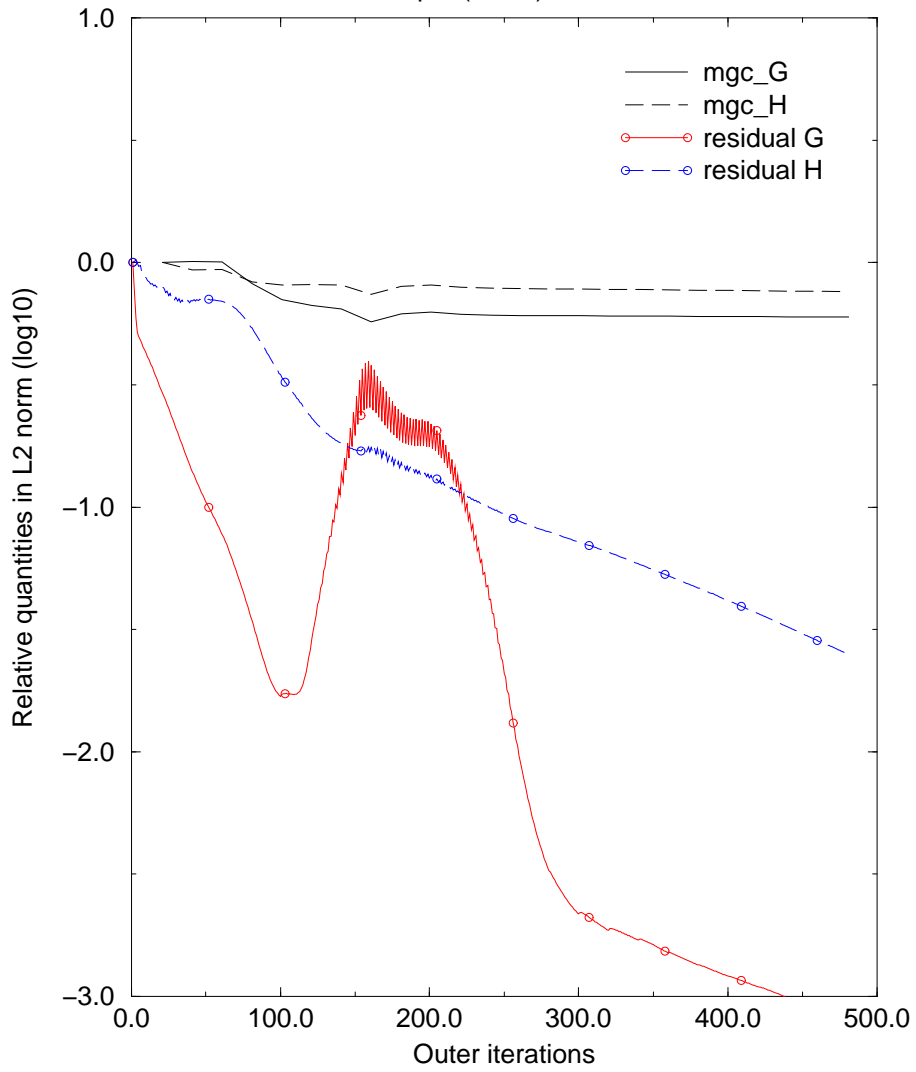
Figure 6: Residual and LDC convergence history, global domain
