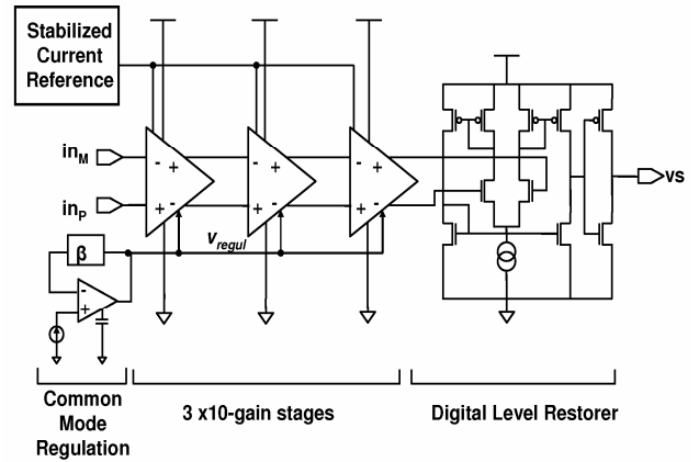
Fig. 6. Principle of the comparator.
