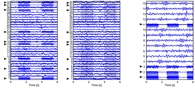
(a) Sources estimated by S-AAS before (left) and after (right) additional F-AAS (b) Sources estimated by ST-AAS
