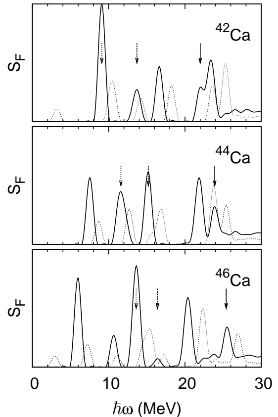
FIG. 4: Strength distributions of the two-neutron pair transfer operator \bar{F} for ^{42,44,46}\text{Ca} (in arbitrary units with the same scale on each plot). TDHFB results (solid lines) and the unperturbed approximation (dotted lines) are shown. The arrows indicate the 1d_{5/2} (solid), 2s_{1/2} (dashed) and 1d_{3/2} (dotted) two deep-hole states.
