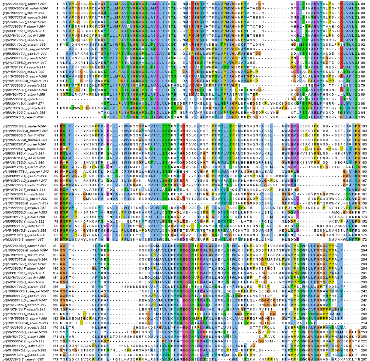
Figure S4. Alignment of PAC1 and PAC2
