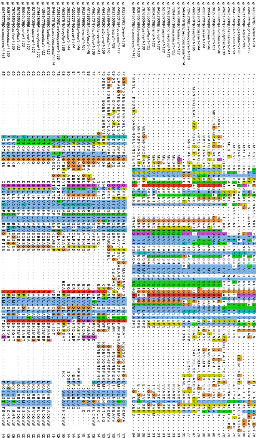
Fig S6. Alignment of PAC3 and PAC4 An initial profile containing S. cerevisiae close homologs was used as a seed for the PSI-BLAST search procedure ran on the nr database (version December 2006). After 3 iterations the search converged with a multiple sequence alignment containing homologs from A. gossypii , C. glabrata , K. lactis , C. albicans , D. hansenii (e-value = 10 -10 ). This first alignment correspond to profile A. A sequence from Y. lipolytica (XP_505861.1) was found with an e-value of 40 among the non significant matches of the last PSI-BLAST iteration. Starting a PSI-BLAST search from this sequence, a set of 21 homologs (corresponding to profile B) could be recovered after 6 iterations, including a human homolog of the Y. lipolytica sequence. The Hhssearch algorithm [Soding-1 Bioinformatics (2005) 21(7):951-60.] was used together with secondary structures predicted using PSIPRED [Jones DT, J Mol Biol. 1999 Sep 17;292(2):195-202.] to evaluate the statistical relevance that both profile A and B contain evolutionarily related sequences. The high probability of 94% and e-value of 3.10 -6 obtained from the Hhssearch comparison supported that both set of sequences are evolutionarily related.
