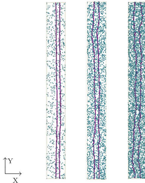
FIG. 1: (color online) View of the (\bar{1}\bar{1}1) glide plane and the dissociated screw dislocation in the Ni(Al) simulated solution at various concentrations: C_{Al} = 2 at. % (lhs), C_{Al} = 6 at. % (center) and C_{Al} = 10 at. % (rhs). The box size is 300 b along Y, 32 b along X and 34 b along Z (orthogonal to this paper sheet). The Shockley partials are colored in violet and the Al atoms in blue. The external shear stress has been fixed to one half of the CRSS.
