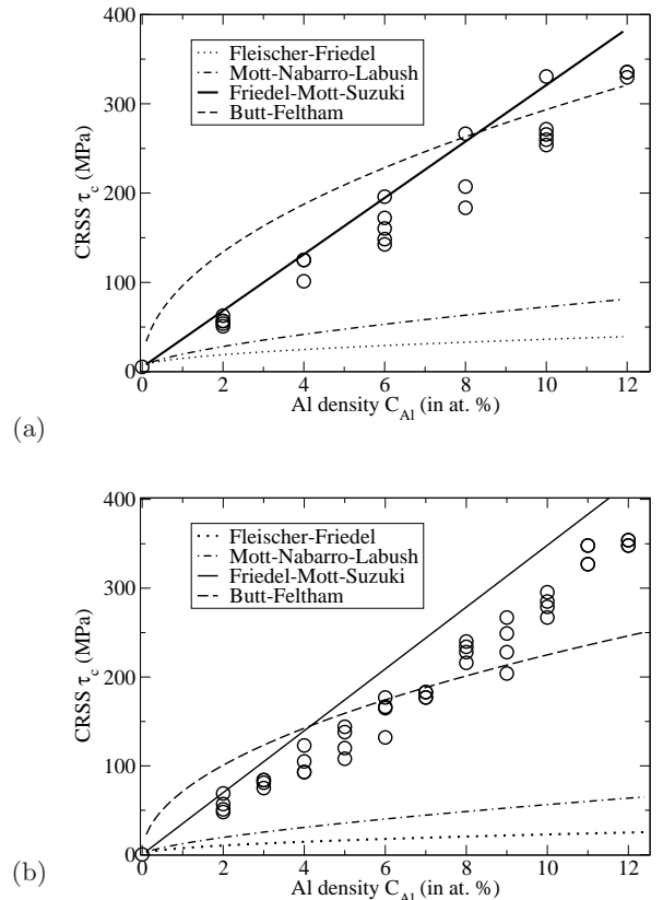
FIG. 2: Variation of the critical resolved shear stress \tau_c for a screw dislocation (a) and for an edge dislocation (b) against the Al concentration C_{Al} computed from the MS simulations with different Al random distributions (symbols). The estimations made with the analytical models have also been reported: Fleischer-Friedel 37 (dotted line), Friedel-Mott-Suzuki 6 (full line), Mott-Nabarro-Labusch 5 (dot-dashed line) and Butt-Feltham 9 (dashed line).
