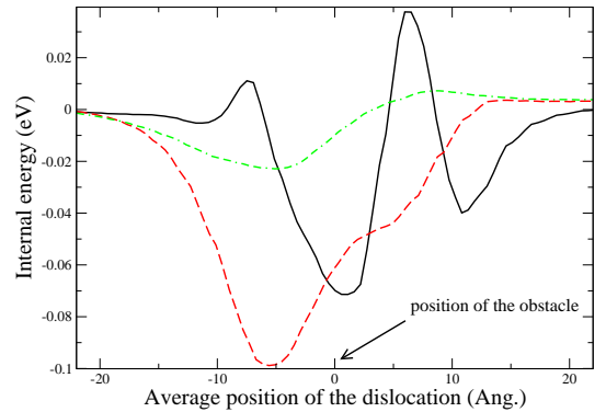
FIG. 3: The internal potential energy for a dissociated screw dislocation against the dislocation obstacle distance. The obstacle is an isolated Al in the ( \bar{1}\bar{1}1 ) planes above the glide plane: the first plane (full line), the second plane (dashed line) and the third one (dot-dashed).
