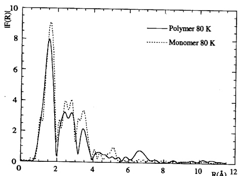
Figure 2-a: Fourier transform modulus in the LS state
