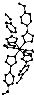
Figure 1-b: monomeric structure
