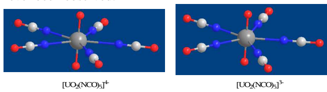
Figure 7: DFT Optimised structures of the U(IV), U(V) and U(VI) isocyanate complexes
