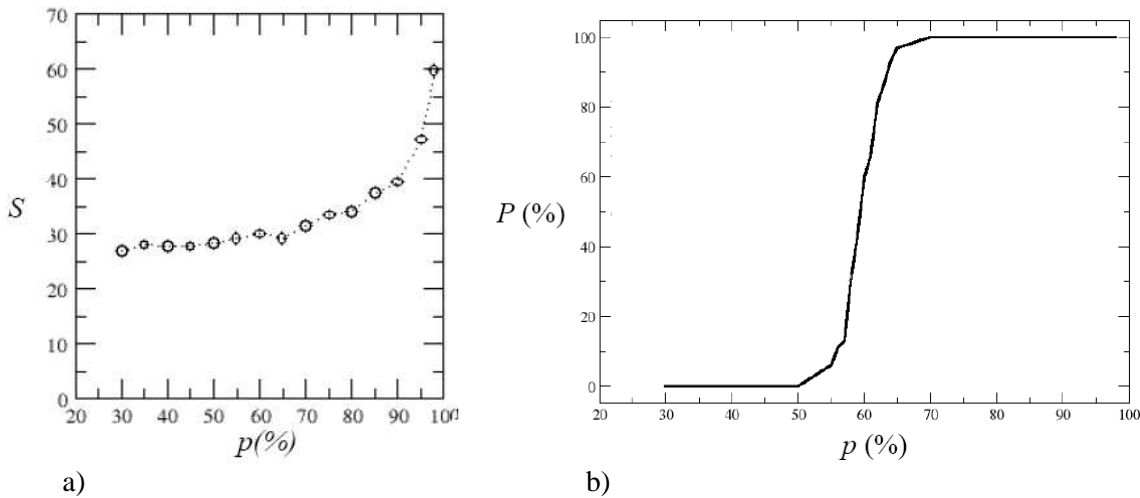
Figure 4. a) Evolution of liquid saturation at breakthrough as a function of hydrophilic pore fraction b) percolation probability of hydrophilic pore subset as a function of hydrophilic pore fraction.
