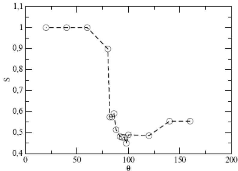
Figure 3. Evolution of overall water saturation at breakthrough, corresponding to patterns shown in Fig.2, as a function of contact angle \theta .
