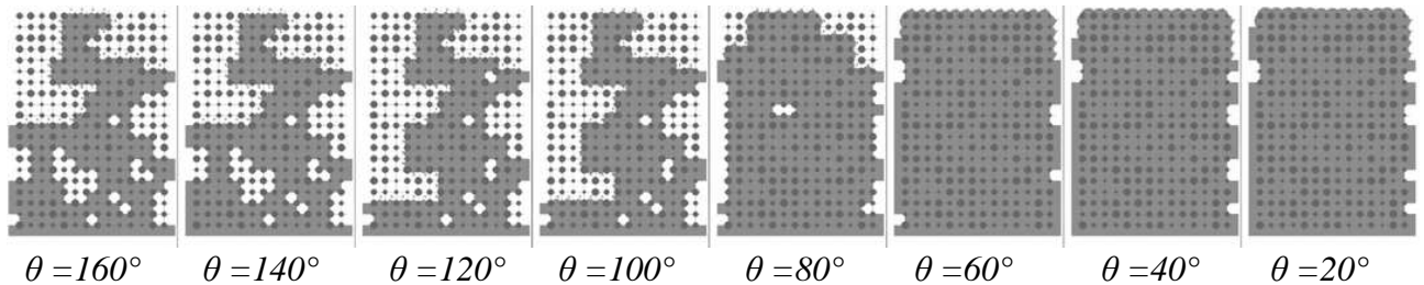
Figure 2. Evolution of invasion pattern at breakthrough in a model fibrous medium as a function of contact angle \theta . Invading phase (liquid water) in grey, displaced phase (air) in white
