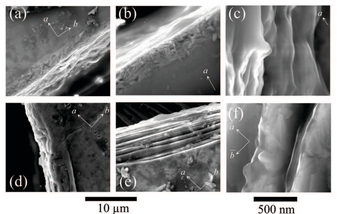
FIG. 3: Scanning electron micrographs of crystal edges cut at 90° (a-c) and at 45° with respect to the principal [100] and [010] crystal axes (d-f). Images (a,b;d,e) have the same magnification, as do images (c,f).
