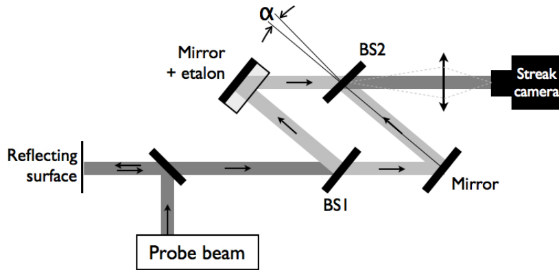
Figure 6.5: Mach Zehnder configuration of the VISAR.
