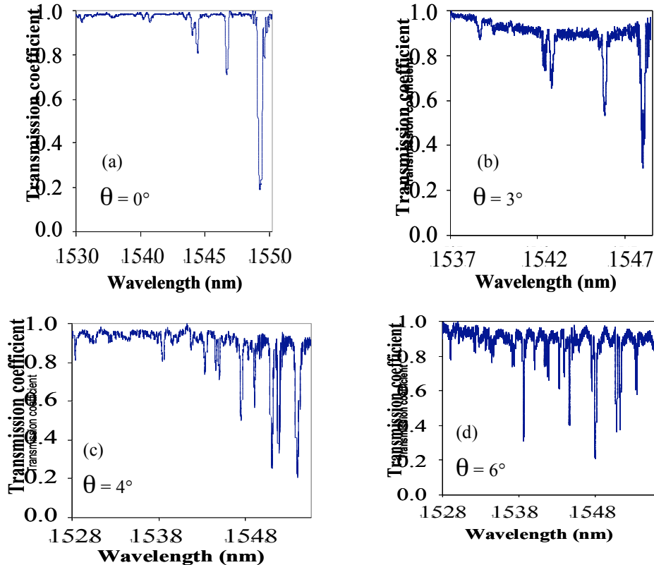
Fig. 6. Transmission spectrum of (a) non-tilted, (b) 3°-tilted, (c) 4°-tilted, (d) 6°-tilted TFBG photowritten in the six-hole fiber.
