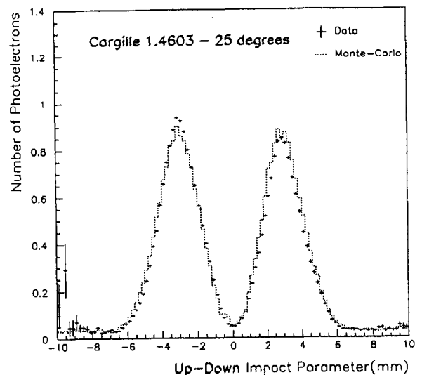
Fig. 6. Amplitude of the signal versus signed impact parameter in the vertical plane, for the sapphire + liquid device at 25^\circ .
