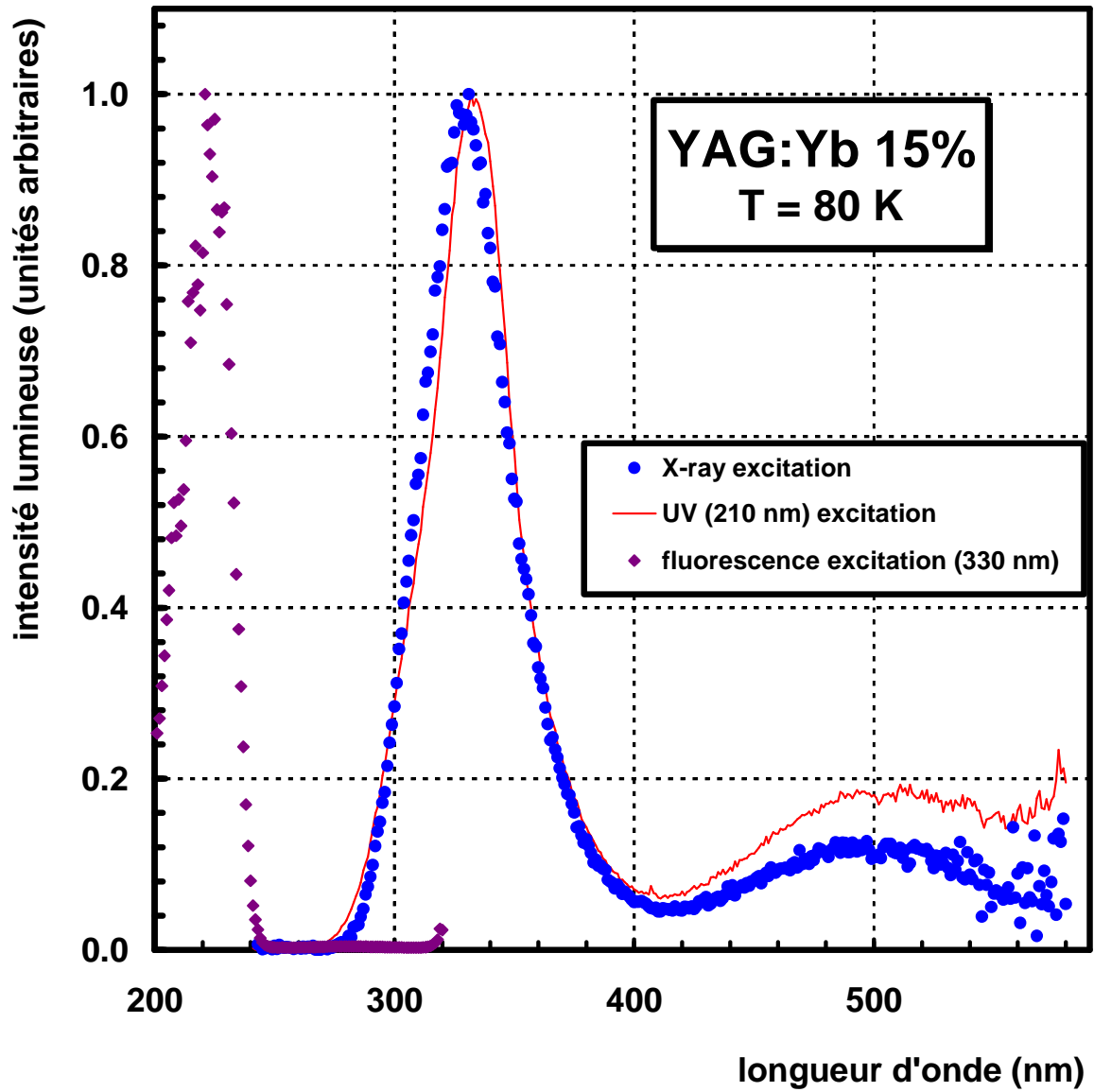
Figure 3-7 : \text{Y}_{2,55}\text{-Yb}_{0,45}\text{Al}_5\text{O}_{12} : Spectres de photo- et radio-luminescence.
