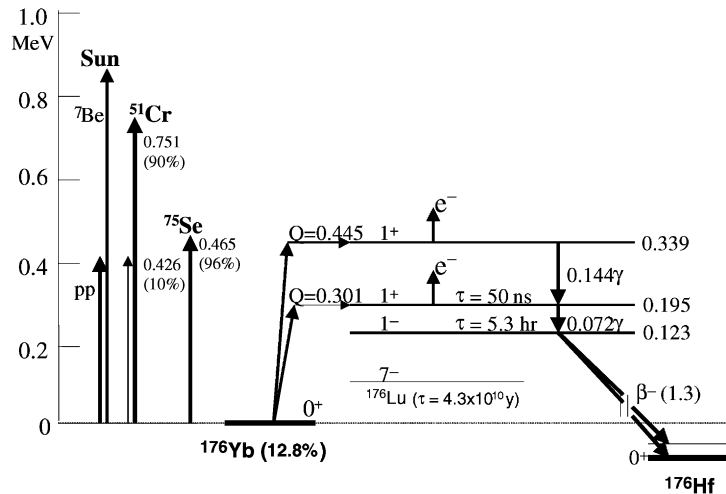
Fig. 2. V_e-^{176}\text{Yb} interaction scheme. Comparison with solar neutrino and ^{51}\text{Cr}/^{75}\text{Se} neutrino sources spectra (on left).
