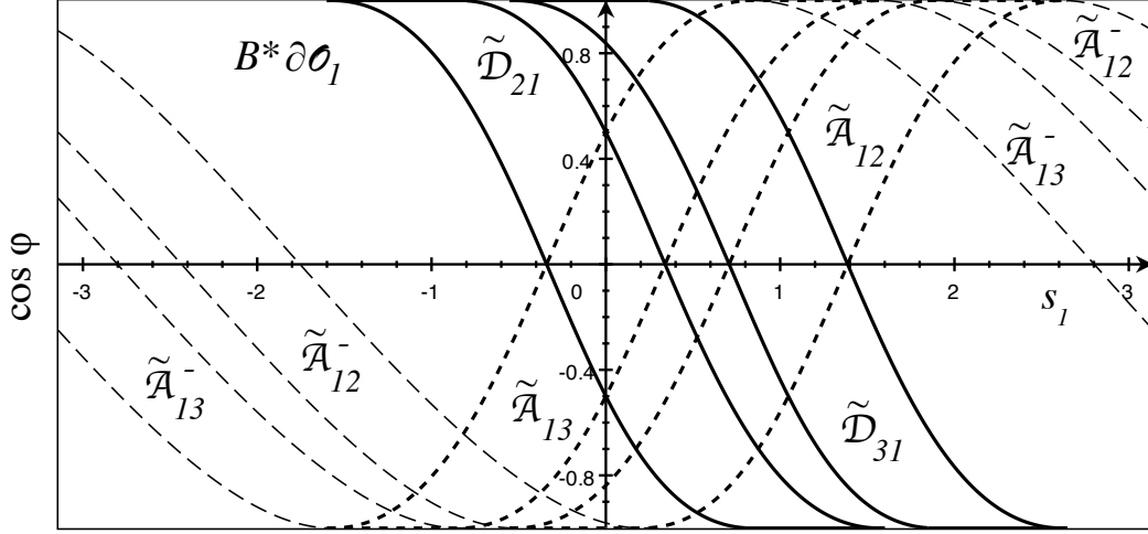
FIGURE 6. (after [32]) Partial boundary phase space B^*\mathcal{O}_1 for the symmetric three disk scattering shown in Fig. 3. We show the boundaries of the departure ( \tilde{D}_{ij} , full lines), arrival ( \tilde{A}_{ij} , dashed lines) and shadow arrival ( \tilde{A}_{ij}^- , long dashed) sets.
