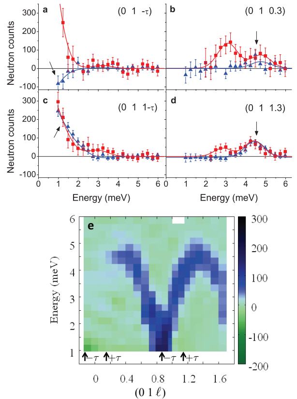
FIG. 3: (a-d) Magnetic scattering S(\vec{Q}, \omega) (red) and chiral contribution C(\vec{Q}, \omega) (blue) as a function of the transfer energy at selected scattering wavevectors (0, 1, \ell) , extracted at 1.5 K by longitudinal neutron polarimetry on the triple-axis spectrometer IN20. The spectral weight is only significant for the branch emerging from the -\tau magnetic satellites. (e) Dispersion of the chiral scattering C(\vec{Q}, \omega) obtained by gathering the measurements at all \ell .
