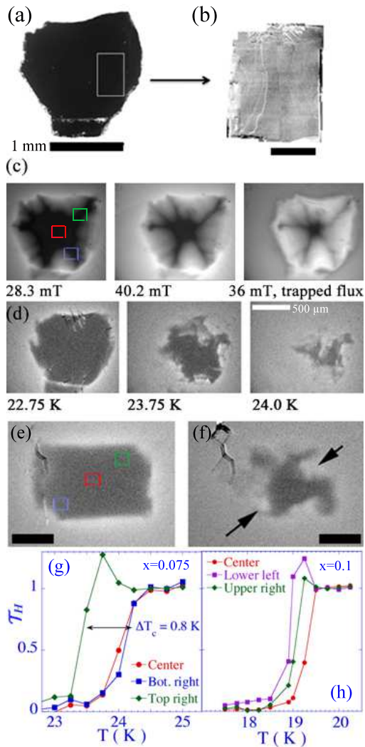
FIG. 1: (Color online) (a) Photograph of \text{Ba}(\text{Fe}_{0.925}\text{Co}_{0.075})_2\text{As}_2 crystal # 2. (b) Scanning electron micrograph of the decorated sample #2.1 cut from the larger crystal #2. (c) Magneto-optical images of \text{Ba}(\text{Fe}_{0.925}\text{Co}_{0.075})_2\text{As}_2 crystal #2 at T = 15 K and indicated values of the applied magnetic field. (d) Differential Magneto-Optical (DMO) images in the vicinity of T_c for \mu_0\Delta H_a = 0.1 mT. (e) DMO image of \text{Ba}(\text{Fe}_{0.9}\text{Co}_{0.1})_2\text{As}_2 crystal #1 at full screening ( T = 17.5 K) and (f) at mid-transition ( T = 19.25 K). The arrows indicate regions of paramagnetic transmittivity at the superconducting transition. (g) Local transmittivity \mathcal{T}_H measured on the three regions of \text{Ba}(\text{Fe}_{0.925}\text{Co}_{0.075})_2\text{As}_2 crystal # 2. (h) \mathcal{T}_H measured on the three regions of \text{Ba}(\text{Fe}_{0.9}\text{Co}_{0.1})_2\text{As}_2 crystal #1 indicated in (e). Scale bars correspond to a length of 100 \mu\text{m} unless indicated otherwise.
