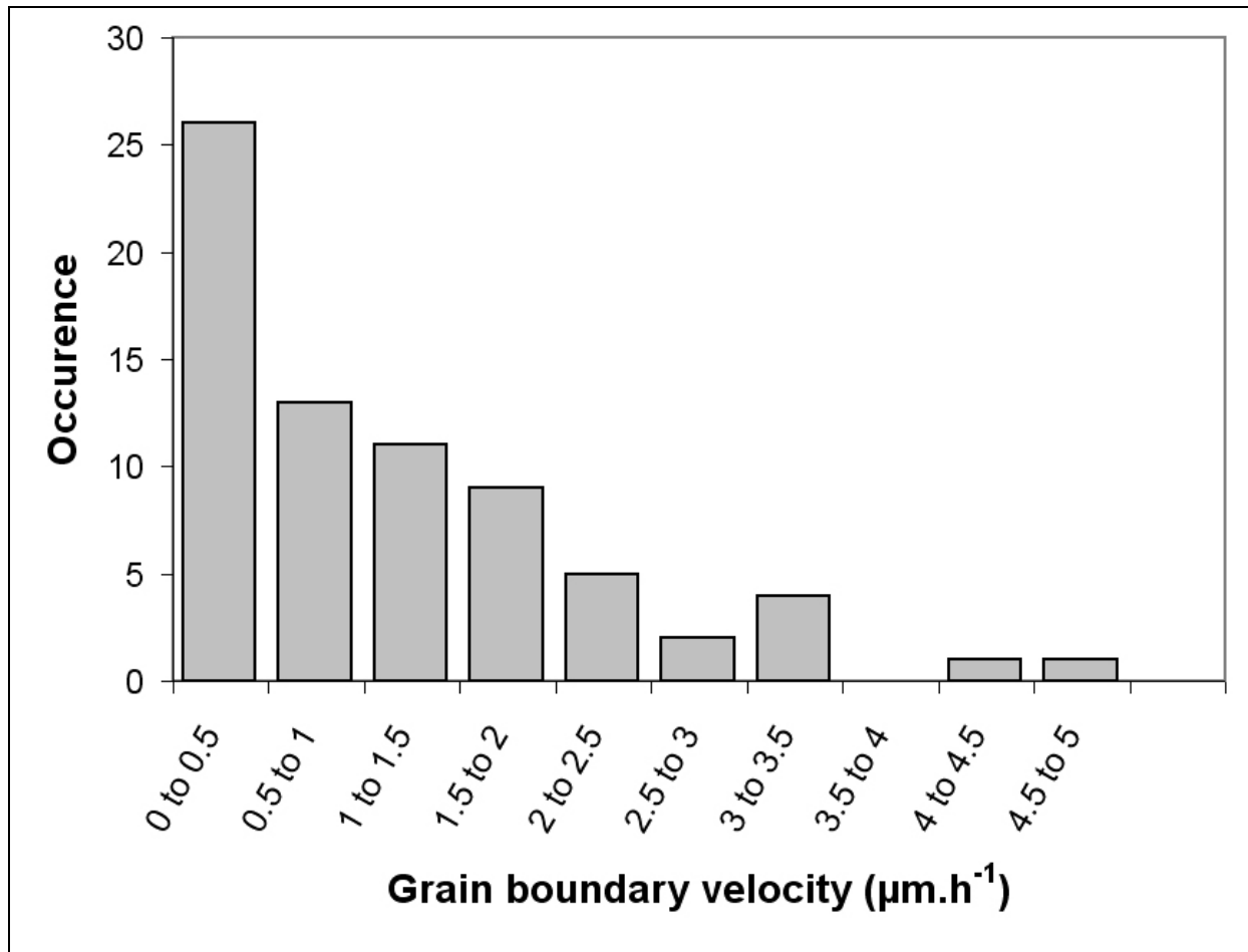
Figure 7 – Distribution of the grain boundary velocity for CeO 2 at T=1400°C
