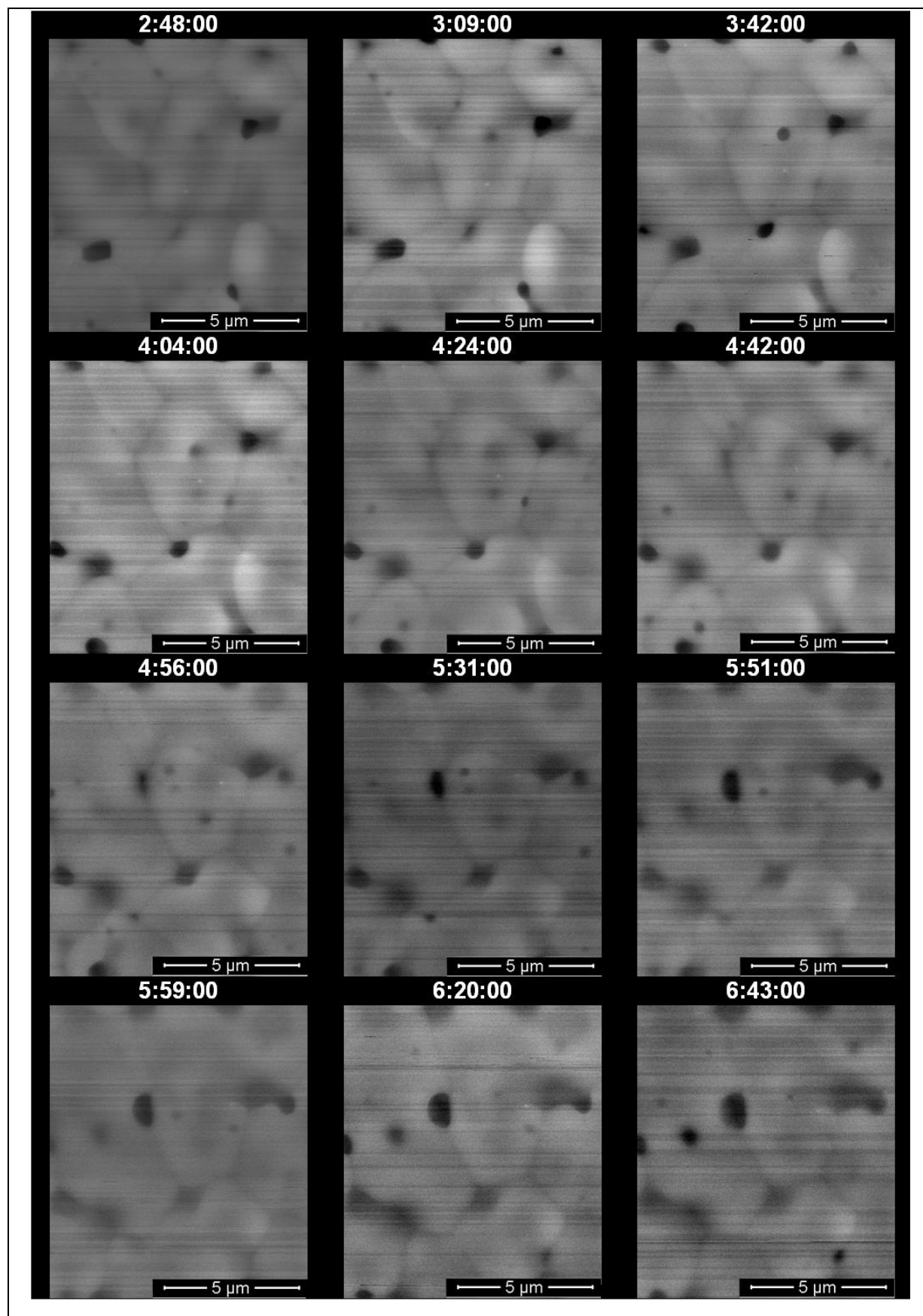
Figure 4 – Selected HT-ESEM images corresponding to different holding times at T=1400°C (heating durations are expressed in h:mn:s). (Please see additional video data for movie)
