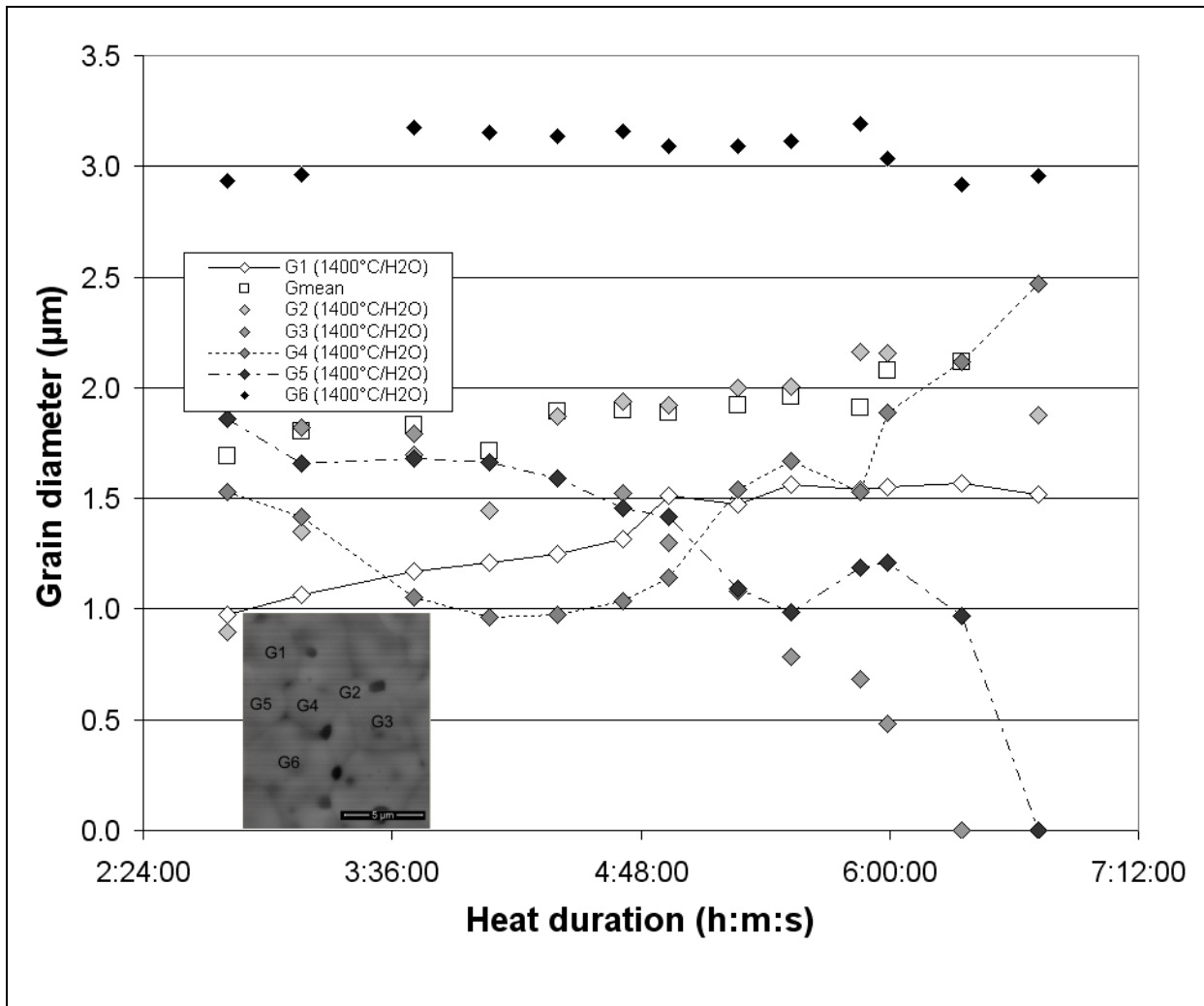
Figure 5 – Variations of local grain sizes versus of heating duration. Locations of the studied grains at the surface of the sample are reported on the inserted image.
