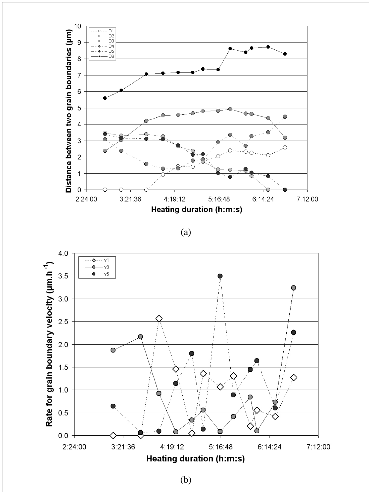
Figure 6 – Determination of the grain boundary velocity (a) Distances between two grain boundaries of a grain. (b) Instantaneous grain boundary velocity (only selected data are reported for easier reading)
