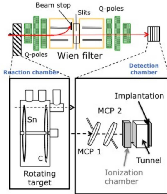
FIG. 1: Experimental setup.
