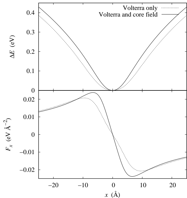
FIG. 9. Variation of the elastic energy, \Delta E , and of the x component of the force \mathbf{F} acting on the dislocations, F_x , with the distance between both dislocations, x , for a screw dipole of height h = 10 \text{ \AA} .
