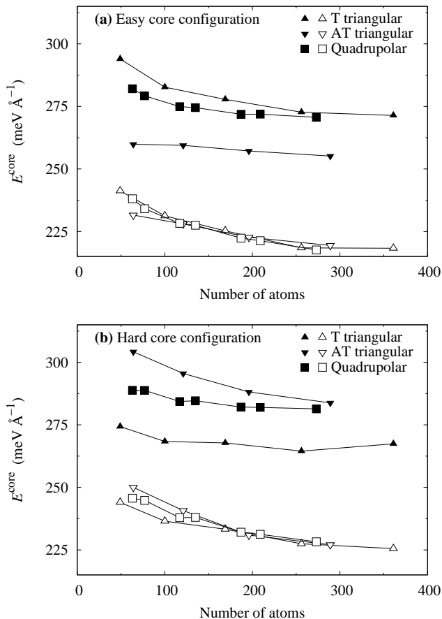
FIG. 5. Core energy of the screw dislocation in the (a) easy and the (b) hard core configuration. Solid symbols correspond to the core energies obtained when only the Volterra field is considered, and open symbols, to the core energies when both the Volterra and the core fields are taken into account ( r_c = 3 \text{ \AA} ).
