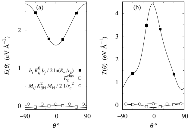
FIG. 6. Elastic contributions [Eq. (5)] to the dislocation (a) line energy E(\theta) and (b) line tension T(\theta) = E(\theta) + d^2E(\theta)/d\theta^2 as a function of the dislocation character \theta in the \{110\} glide plane. \theta = 0 for the screw orientation.
