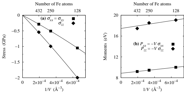
FIG. 12. Variation of the stress \sigma_{ij} and of the corresponding dipolar tensor P_{ij} with the inverse of the volume V of a unit cell containing one C atom in a [001] variant embedded in an Fe matrix. Symbols correspond to ab initio calculations and solid lines to Eq. (B1) and (B2).
