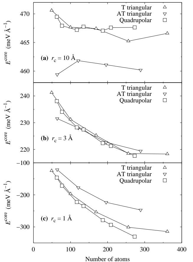
FIG. 11. Core energy of the screw dislocation in the easy core configuration for different core radii: (a) r_c = 10 \text{ \AA} , (b) r_c = 3 \text{ \AA} , and (c) r_c = 1 \text{ \AA} . Both the Volterra and the core fields have been considered in the elastic energy.
