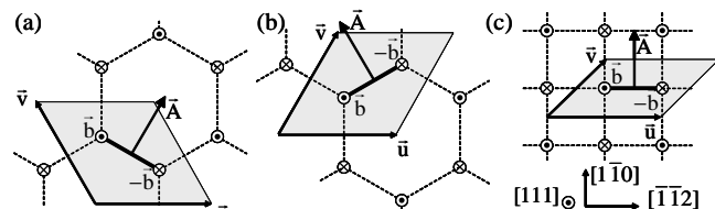
FIG. 1. Screw dislocation periodic arrangements used for ab initio calculations: (a) T and (b) AT triangular arrangements, (c) quadrupolar arrangement. \mathbf{u} and \mathbf{v} are the unit cell periodicity vectors, and \mathbf{A} the dipole cut vector. In all cases, the Burgers vector \mathbf{b} = \frac{1}{2}a_0 [111] for easy, and -\frac{1}{2}a_0 [111] for hard core configuration.
