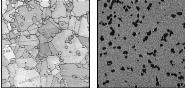
(a) Udimit 720: quality image SEM/EBSD
