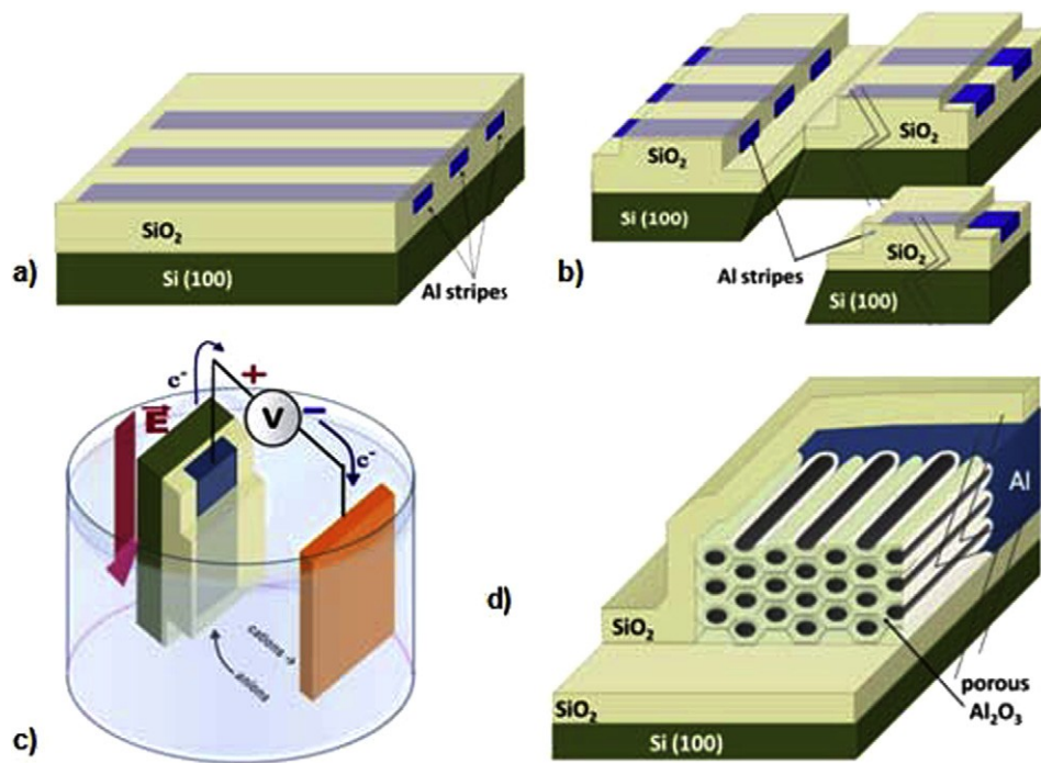
Fig. 3. Principle of the method developed for synthesising lateral porous alumina templates. (a): Al stripes deposited on an oxidised Si wafer are capped with an insulating layer (e.g., \text{SiO}_2 ). (b): The capped Al stripes are made individual by photolithography and cleavage of the substrate. (c): Anodic oxidation of the tip of an individual Al stripe. (d): Schematic structure of the lateral porous alumina membrane at the tip of the Al stripe, after anodic oxidation.
