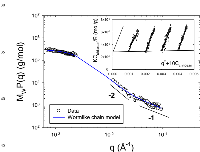
Fig. 1 Combined static light scattering and SANS spectra for a 0.1g/l chitosan solution. To superimpose both techniques we plot M_W P(q) as a function of q . The continuous line represents the fit of the data with a wormlike chain model (see ESI). The Zimm plot of chitosan is presented in the inset.
