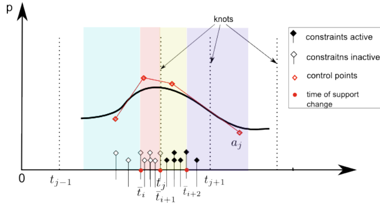
Figure 5.9: There are less constraints when the knot interval becomes smaller.
