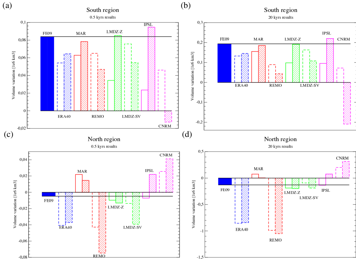
Fig. 9. Regional volume difference (simulated volume minus initial volume, being 1.10 and 0.46 \cdot 10^6 \text{ km}^3 for north and south, respectively) for each model run. Empty bars correspond to the standard volume difference ( dV_i ) and hatched bars correspond to the volume difference computed with the precipitation in each model replaced by the Ettema et al. (2009) precipitation map ( dV'_i ). The first solid bar is the simulated reference volume difference ( dV_0 , FE09). The upper panel corresponds to the south region (latitudes lower than 68^\circ\text{N} ) at 0.5 kyr (a) and 20 kyr (b), and the lower panel corresponds to the north region (latitudes greater than 75^\circ\text{N} ) at 0.5 kyr (c) and 20 kyr (d).
