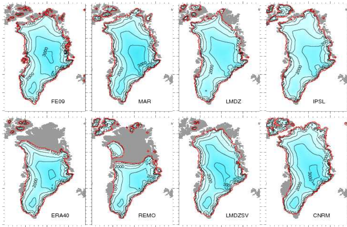
Fig. 5. Simulated ice sheet topography at the end of the 20-kyr constant climate forcing model run.
