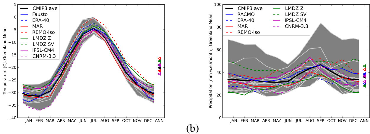
Fig. 2. Greenland (land points) mean seasonal cycle of near surface air temperature (in ^{\circ}\text{C} , left panel) and precipitation (in millimetres of water equivalent per month, right panel) for the 8 atmospheric forcing fields used in this study (coloured lines). For FE09, temperature is representative for the 1996–2006 period (Fausto et al., 2009) and precipitation for the 1958–2009 period (Ettema et al., 2009). For the other forcing fields, climatological means are evaluated on the 1980–1999 period. Annual mean values are represented by triangles on the right. The grey, shaded area is the spread of 12 CMIP-3 models. Light grey and black lines, respectively, represent individual models and their means.
