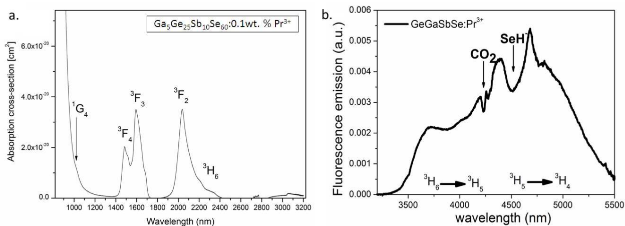
Figure 5. (a) Absorption cross-coefficient of Pr 3+ : GaGeSbSe glass; (b) Fluorescence emission of Pr 3+ :GaGeSbSe fiber excited at 2 μm. Such fibers, emitting in the mid-IR are very promising in view of detecting chemical species absorbing in the 3.5 to 5.5 μm range.
