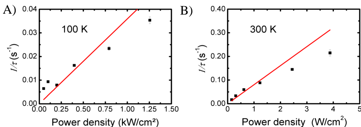
Figure 2.42) Photoactivation of Padron occurs via a 1-photon absorption process at low to room temperature. (A) At 100 K, the photoactivation rate reports on the buildup of I_{\text{cis}} (actinic laser at 532 nm). (B) At room temperature, the rate reports on the buildup of AB_{\text{cis}} (actinic laser at 488 nm).
