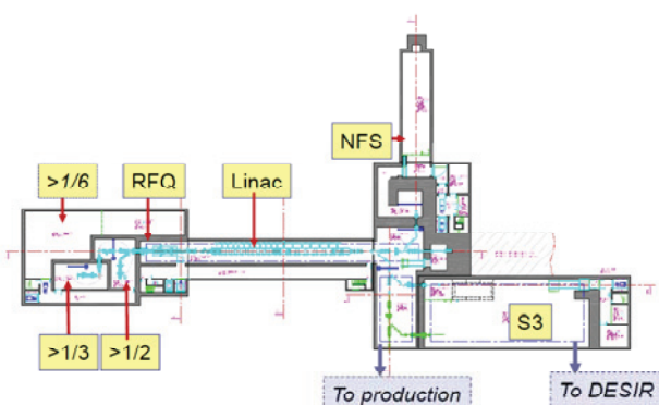
Figure 1: The Spiral2 accelerator phase.
