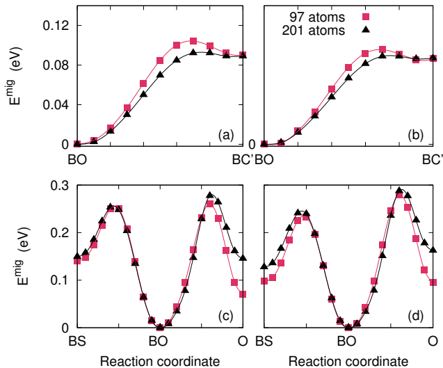
FIG. 4. Migration pathways of Zr SIA calculated with the NEB method, between the BO and BC' configurations and between the BS, BO and O configurations: (a), (c) uncorrected and (b), (d) corrected results.
