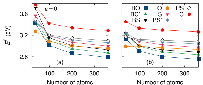
FIG. 3. Uncorrected (a) and corrected (b) Zr SIAs formation energies E^f of the stable configurations versus the number of atoms for \varepsilon = 0 calculations.
