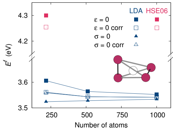
FIG. 6. Vacancy formation energy E^f in silicon calculated with the LDA and HSE06 functionals, either for fixed periodicity vectors ( \epsilon = 0 ) or at zero stress ( \sigma = 0 ). Filled symbols refer to the ab initio uncorrected results and open symbols to the results corrected by the elastic model. The vacancy configuration is displayed in the inset: the white sphere corresponds to the empty lattice site and the purple spheres represent its first nearest neighbors.
