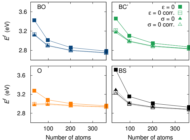
FIG. 2. Formation energies E^f of the four most stable SIAs in Zr versus supercell size. Filled symbols refer to ab initio uncorrected results and open symbols to the results corrected by the elastic model. The periodicity vectors of the supercell have been either kept fixed (square) or relaxed (triangles) in the ab initio calculations.
