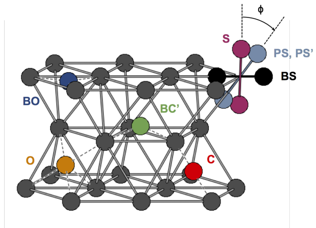
FIG. 1. Structures of the stable SIA configurations in hcp Zr: Octahedral (O), basal octahedral (BO), split dumbbell (S), basal split dumbbell (BS), crowdion (C) and buckled basal crowdion (BC'). PS and PS' are obtained by a rotation of angle \phi = 30^\circ and 50^\circ of S in the prismatic plane. 26
