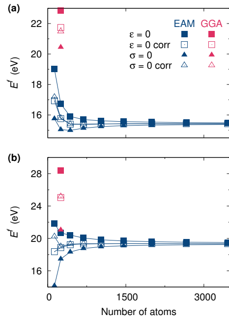
FIG. 5. Formation energy of a SIA cluster containing eight interstitials in bcc iron calculated for fixed periodicity vectors ( \varepsilon = 0 ) or at zero stress ( \sigma = 0 ) for different sizes of the simulation cell: (a) C15 aggregate and (b) parallel-dumbbell configuration with a \langle 111 \rangle orientation. Atomistic simulations are performed either with the M07 empirical potential 7 (EAM) or with ab initio calculations (GGA). Filled symbols refer to uncorrected results and open symbols to the results corrected by the elastic model.
